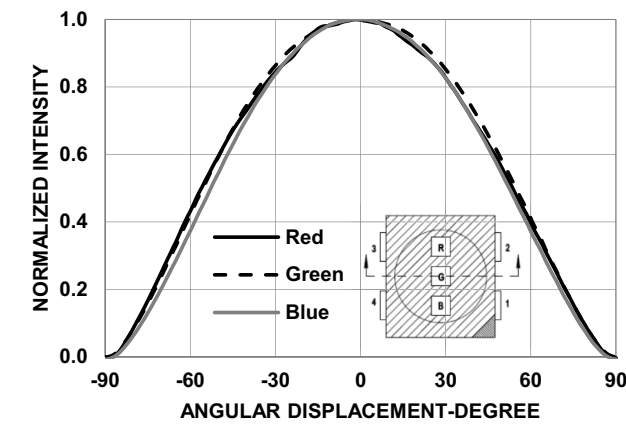
Figure 10: Radiation Pattern for X-axis
