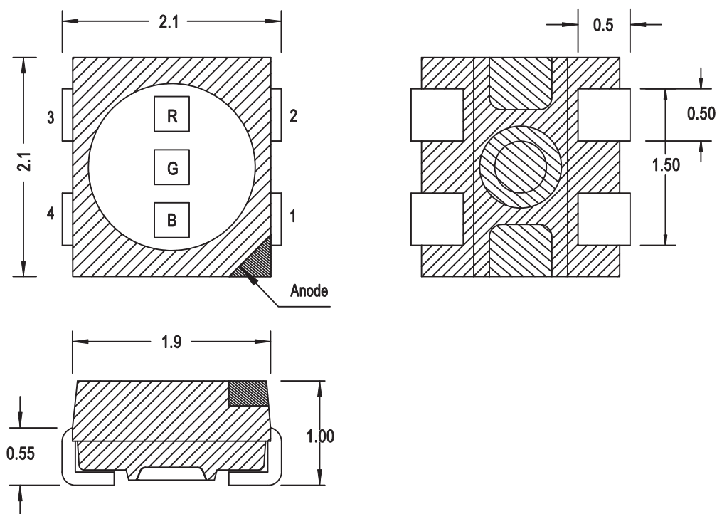
Figure 1: Package Drawing
