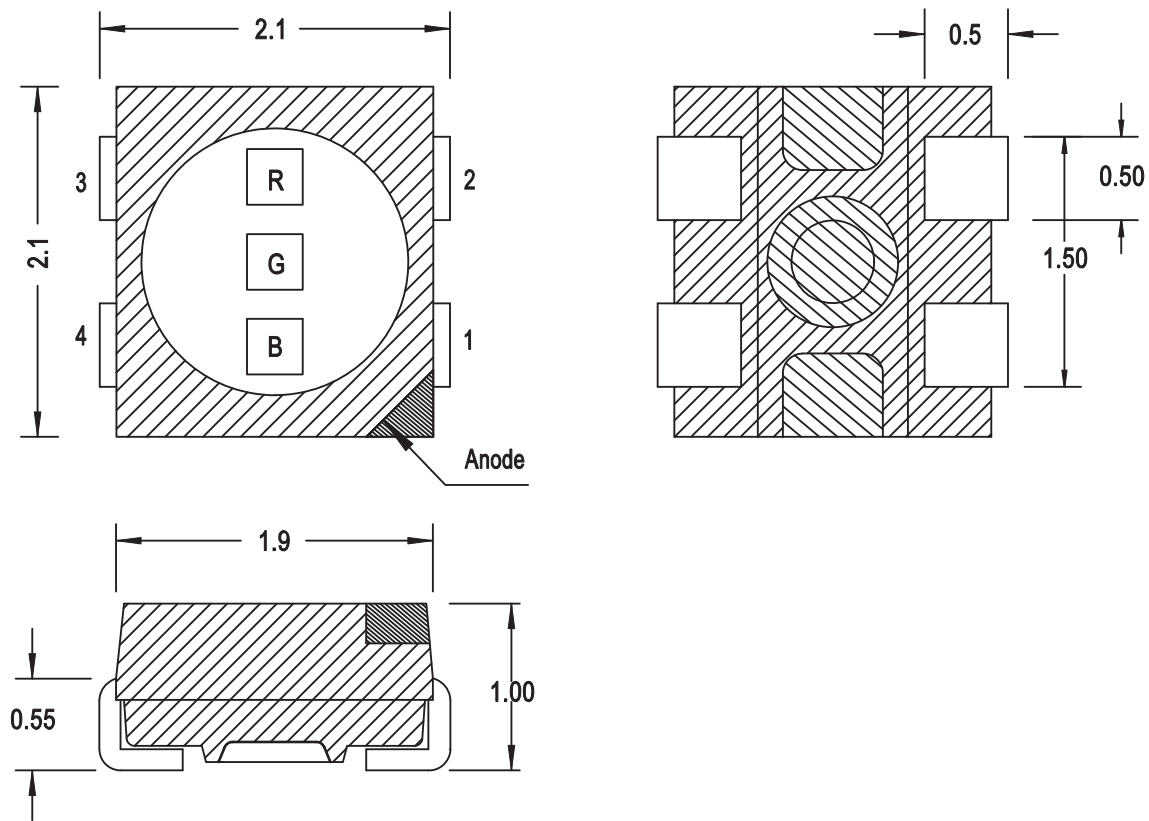
Figure 1: Package Drawing
