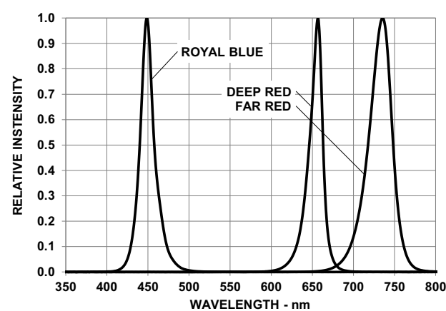
Figure 4: Spectral Power Distribution for Far Red, Deep Red, and Royal Blue
