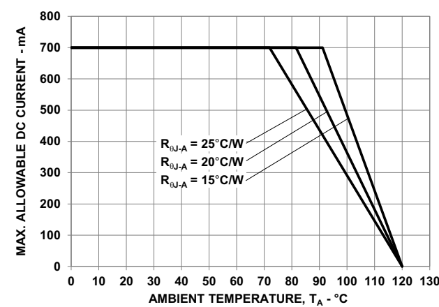
Figure 16: Maximum Forward Current vs. Ambient Temperature for AlInGaP
