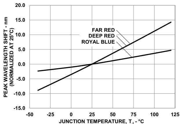
Figure 14: Peak Wavelength Shift vs. Junction Temperature
