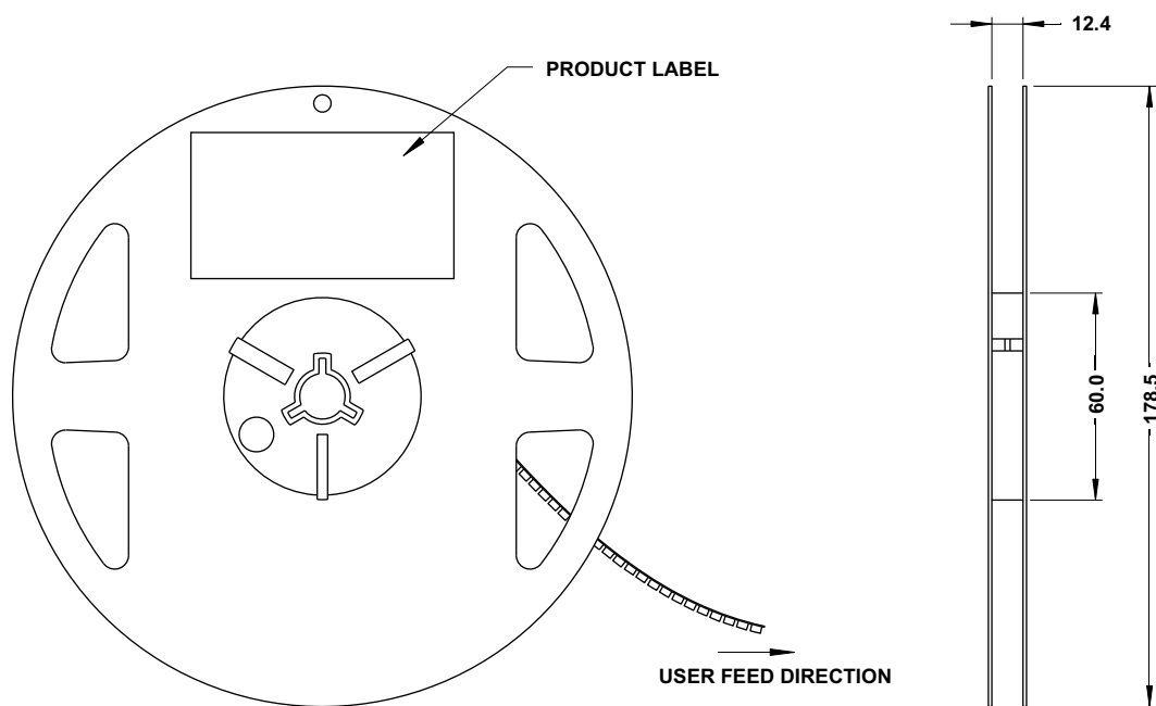
Figure 20: Reel Dimensions
