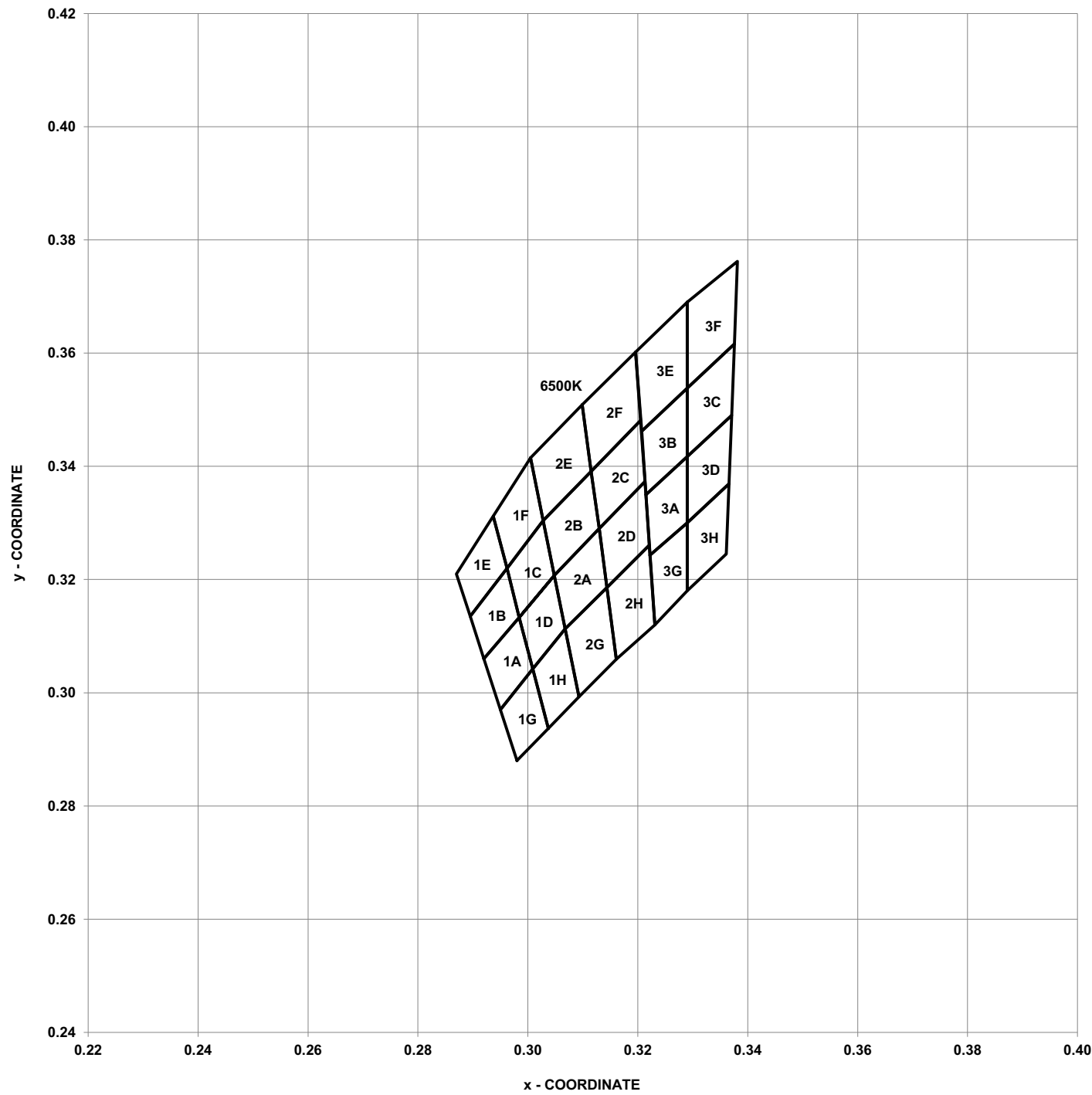
Figure 2: Chromaticity Diagram
