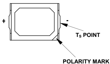
Figure 19: Solder Point Temperature on PCB
