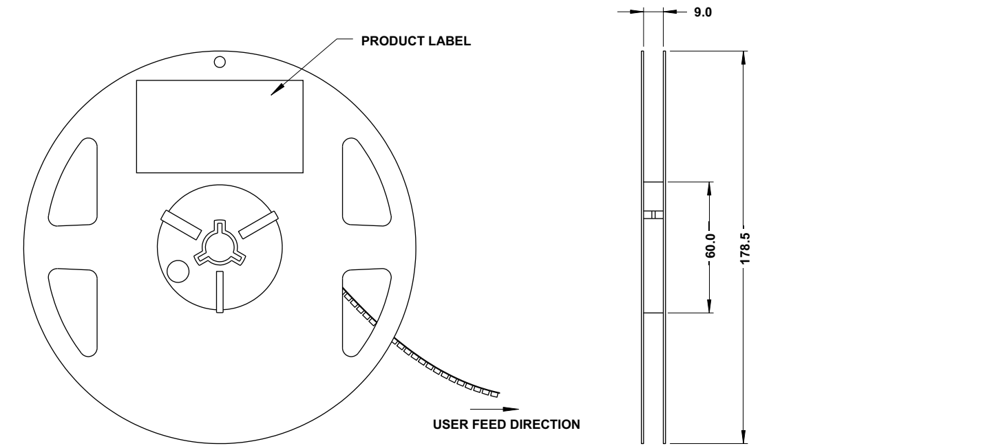
Figure 16: Reel Dimensions
