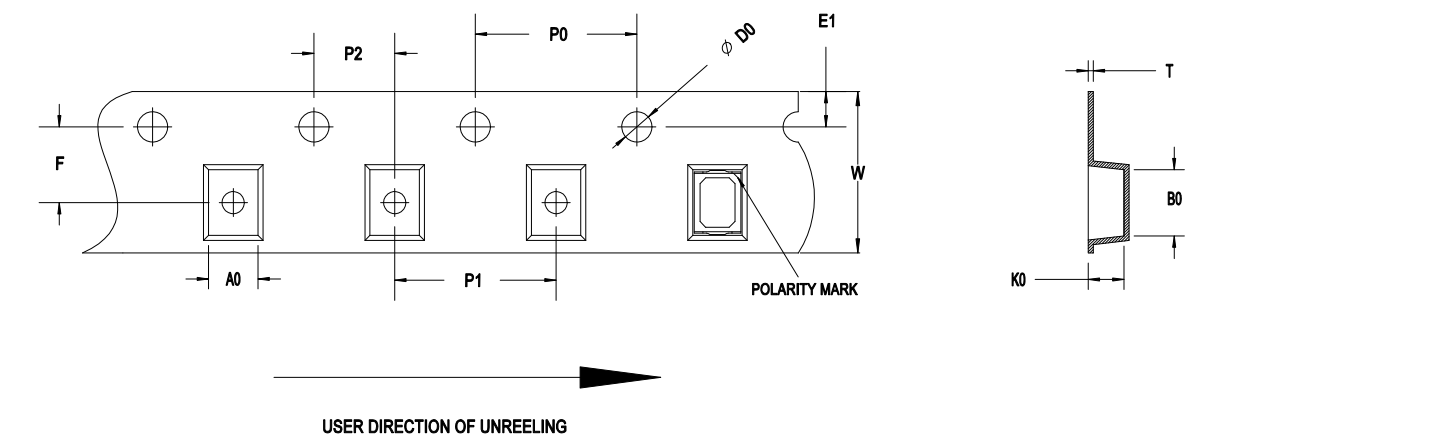
Figure 15: Carrier Tape Dimensions
