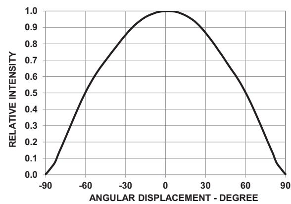
Figure 6: Radiation Pattern
