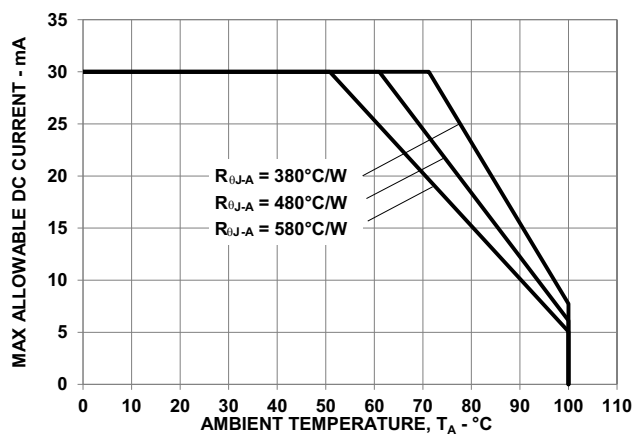
Figure 12: Maximum Forward Current vs. Ambient Temperature. Derated based on T_{JMAX} = 110^{\circ}\text{C}
