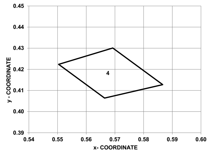
Figure 2: Chromaticity Diagram
