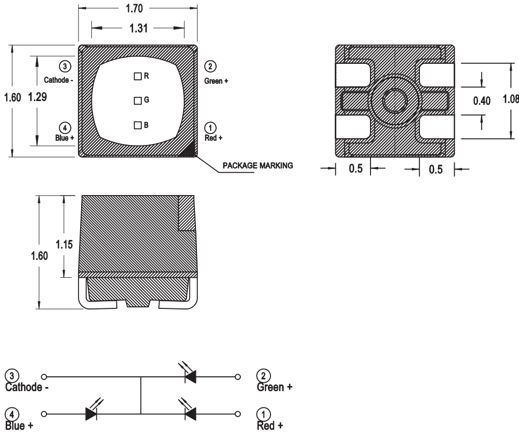
Figure 2: Package Drawing
