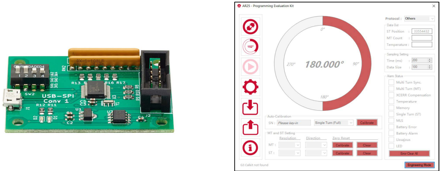
Figure 16: AR25-E01 Calibration Kit and Software User Interface
