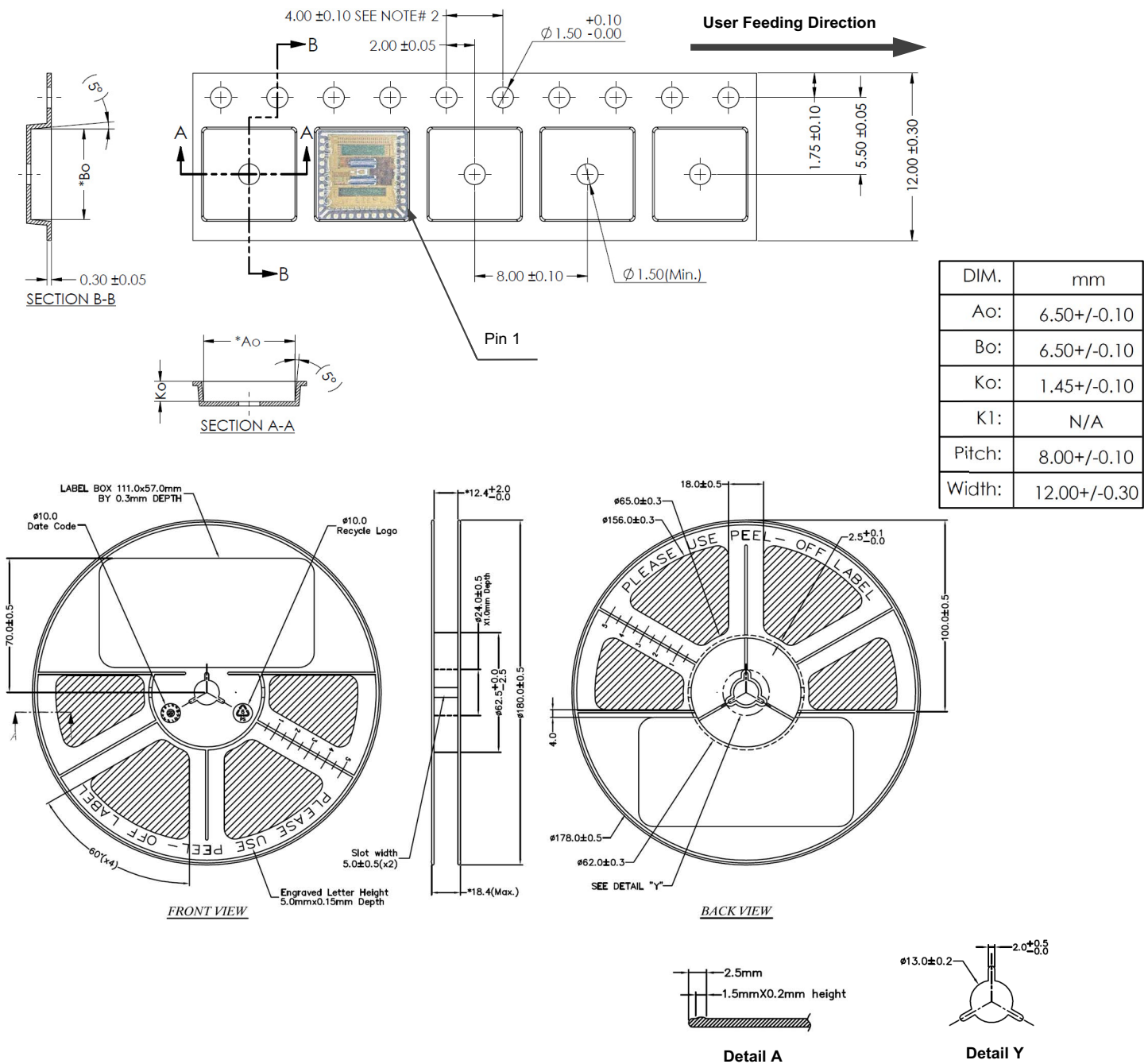
Figure 14: AR25DP Carrier Tape Dimensions
