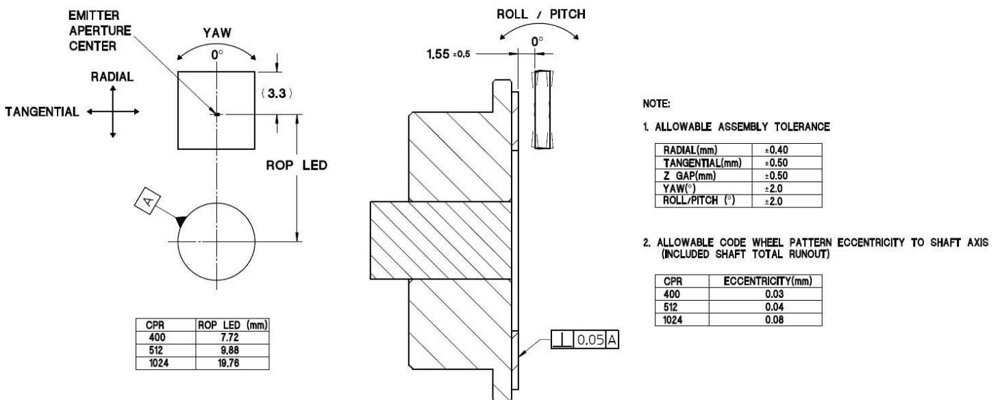
Figure 9: Encoder Mounting Details
