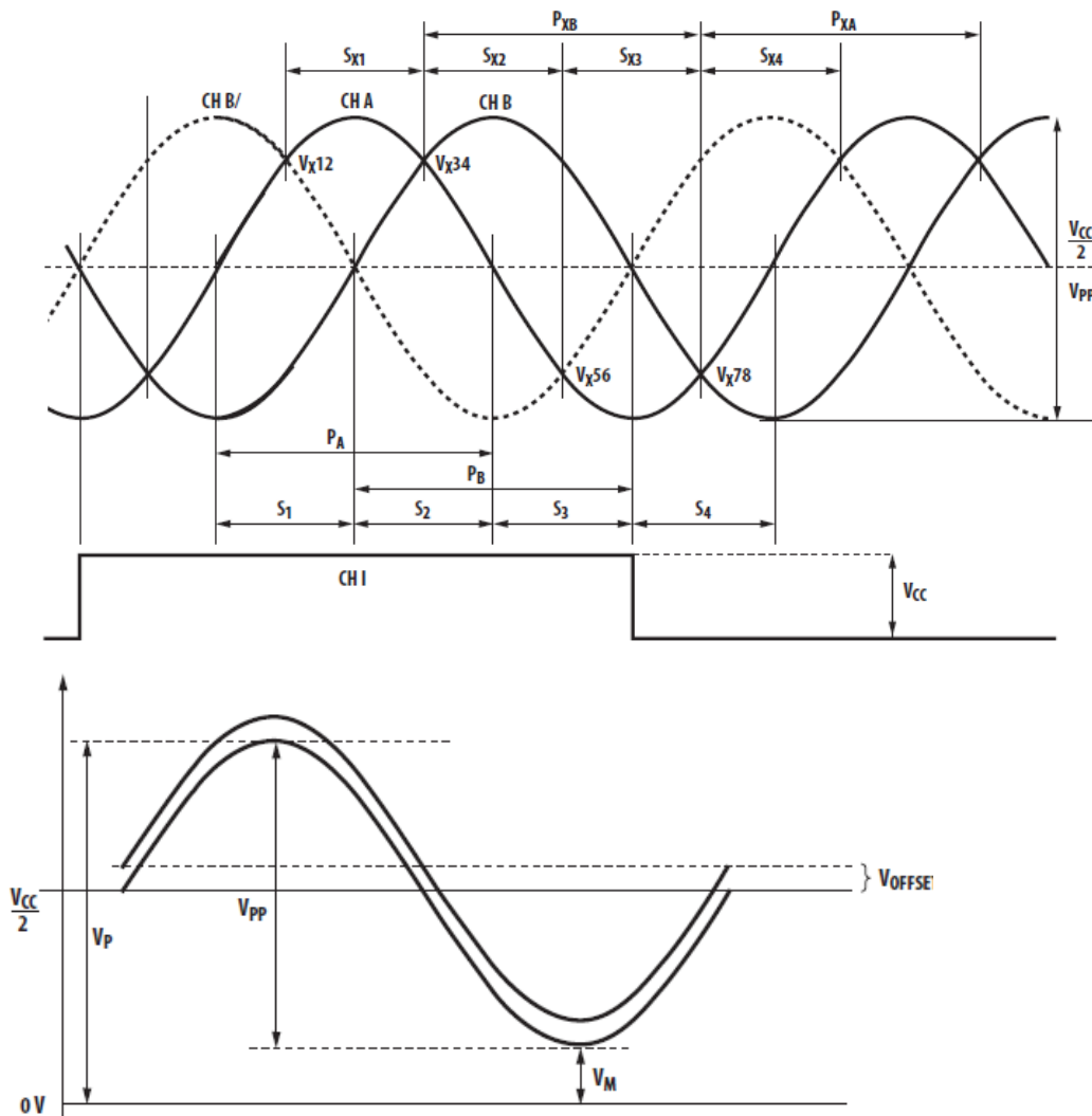
Figure 13: Analog Waveform
