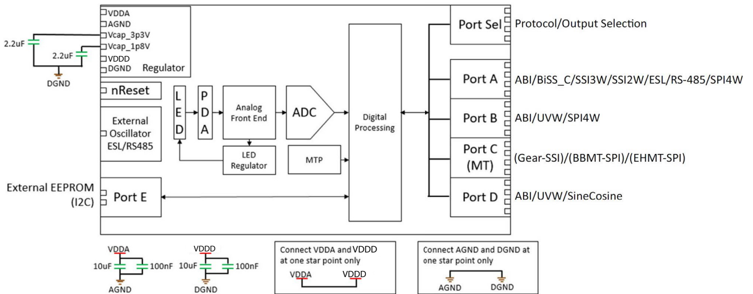
Figure 1: AR25DP Block Diagram
