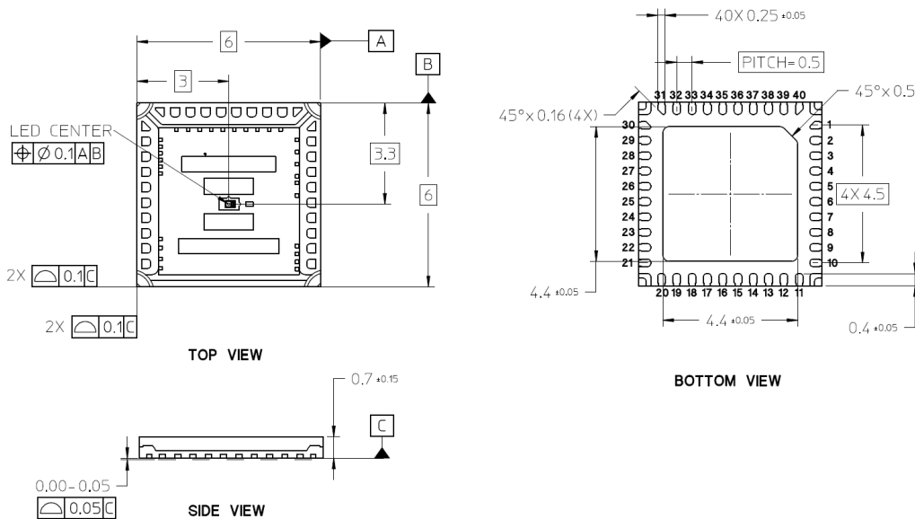
Figure 7: Overall Package Dimensions and Pinout
