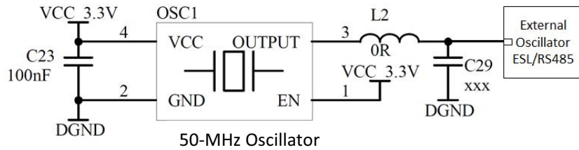
Figure 2: AR25DP External Oscillator Connection Diagram
