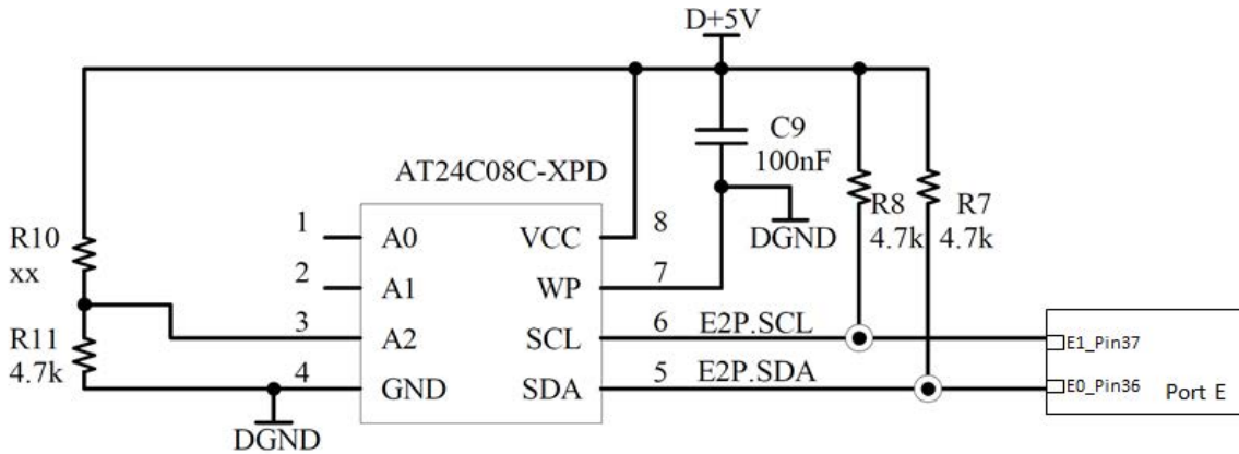
Figure 3: AR25DP External EEPROM Connection Diagram
