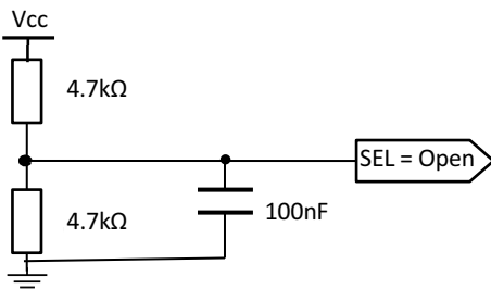
Figure 6: Example of a Voltage Divider Circuit
