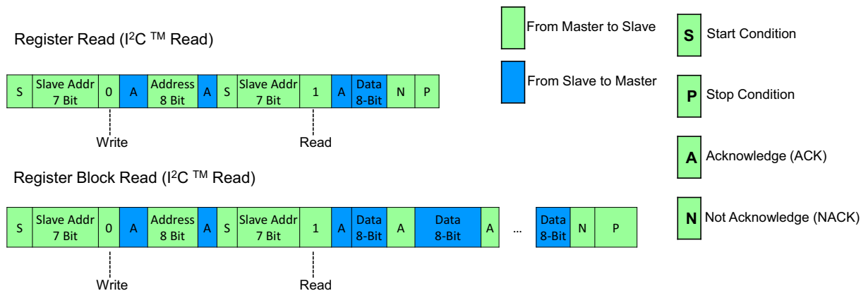
Figure 10: I 2 C Register Read Timing Diagram
