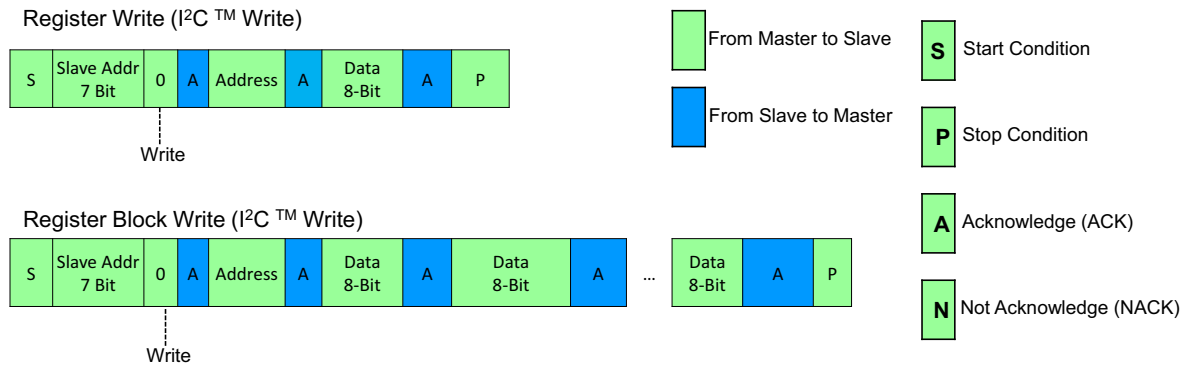
Figure 11: I 2 C Register Write Timing Diagram
