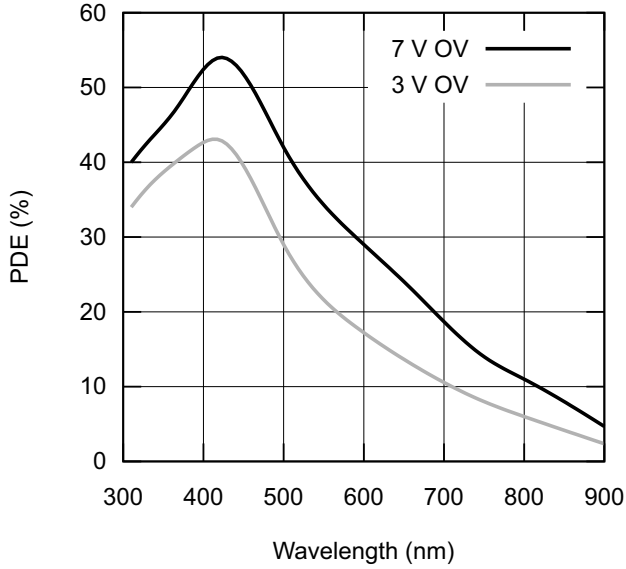
Figure 4: Spectral Sensitivity
