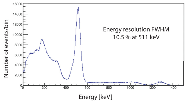
Figure 5: Energy Spectrum with LYSO 3 × 3 × 5 mm 3 Measured with PETSysTOFPET2 ASIC
