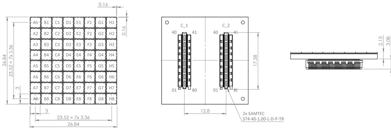
Figure 1: AFBR-S4K33P6425B Dimensions
