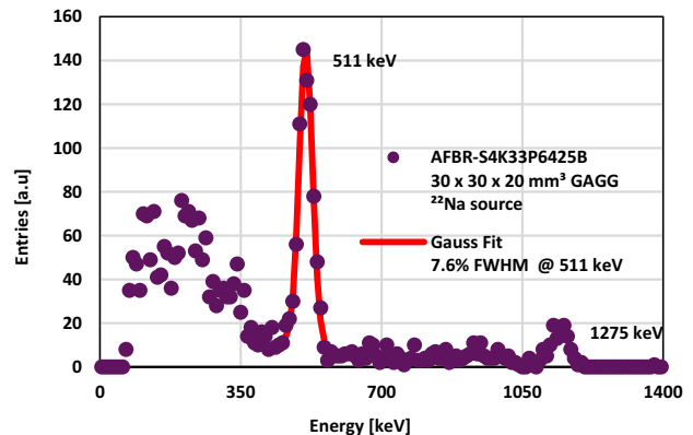
Figure 7: Energy Spectrum with Monolithic GAGG 30 × 30 × 20 mm 3 Measured with Vertilon ISQP582
