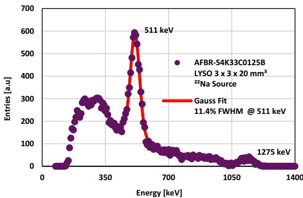
Figure 6: Energy Spectrum with LYSO 3 × 3 × 20 mm 3 Measured with Vertilon ISQP582
