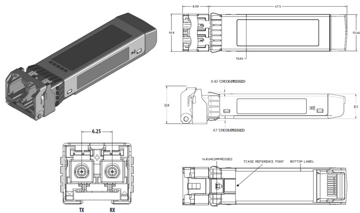
Figure 7: Module Drawing
