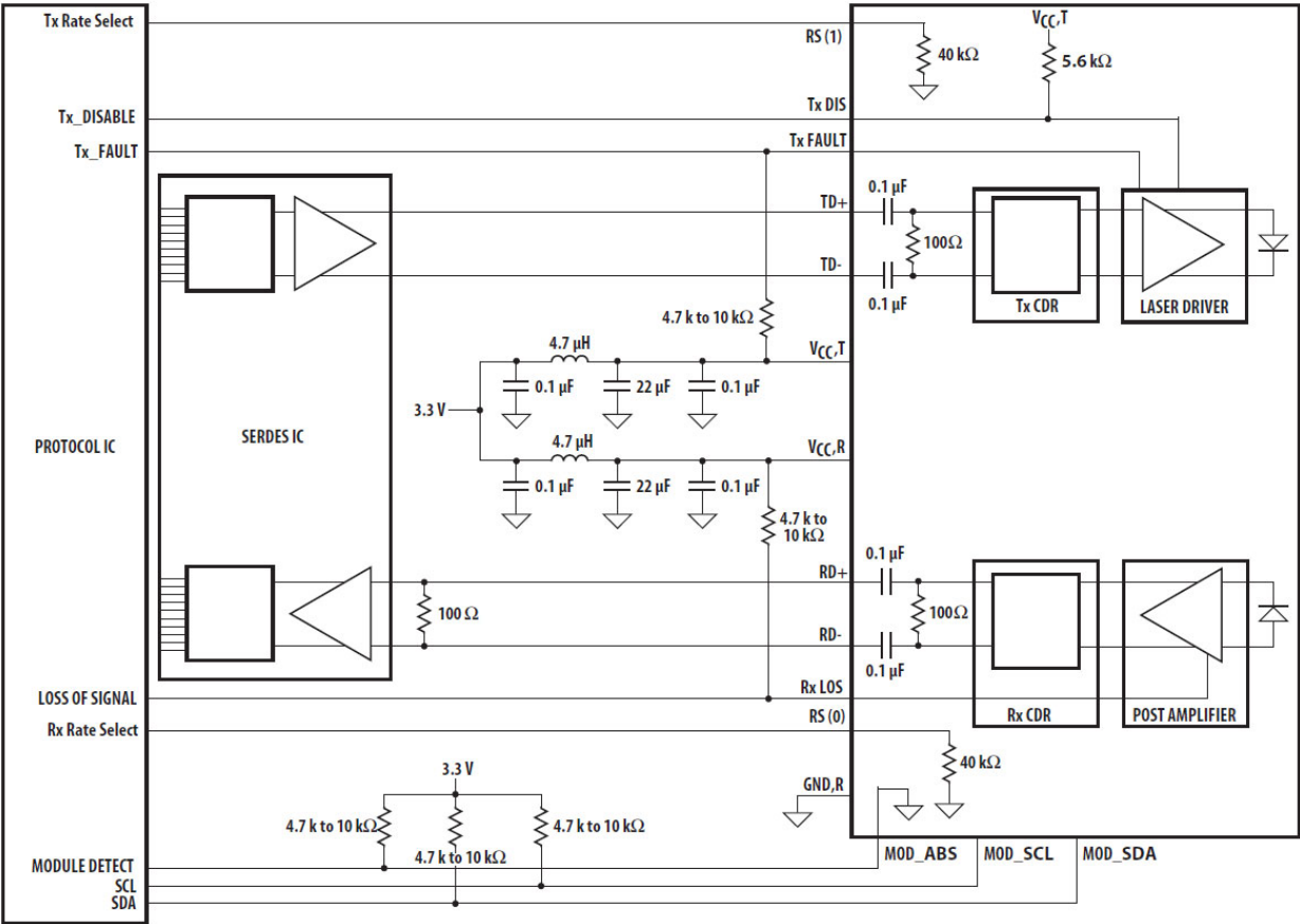
Figure 3: Recommended Power Supply Filter
