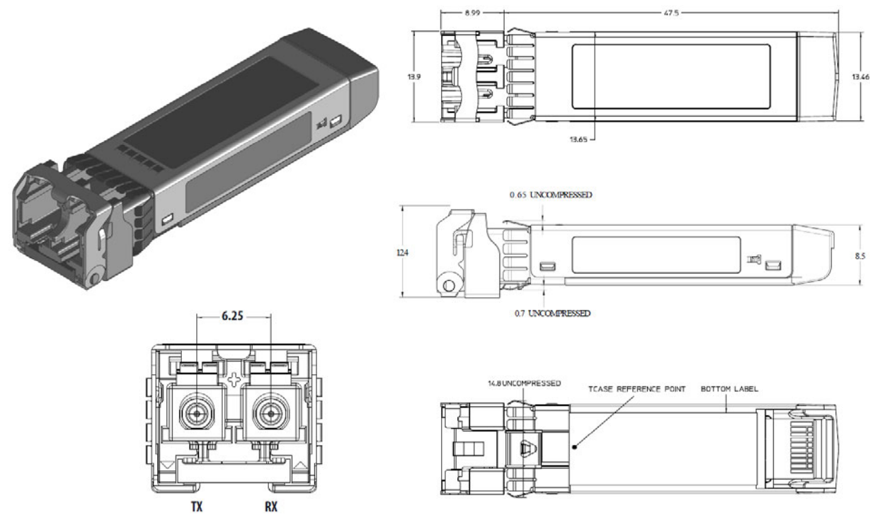
Figure 7: Module Drawing
