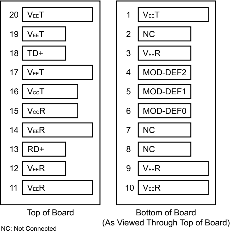
Figure 1: PCB Pin Connection
