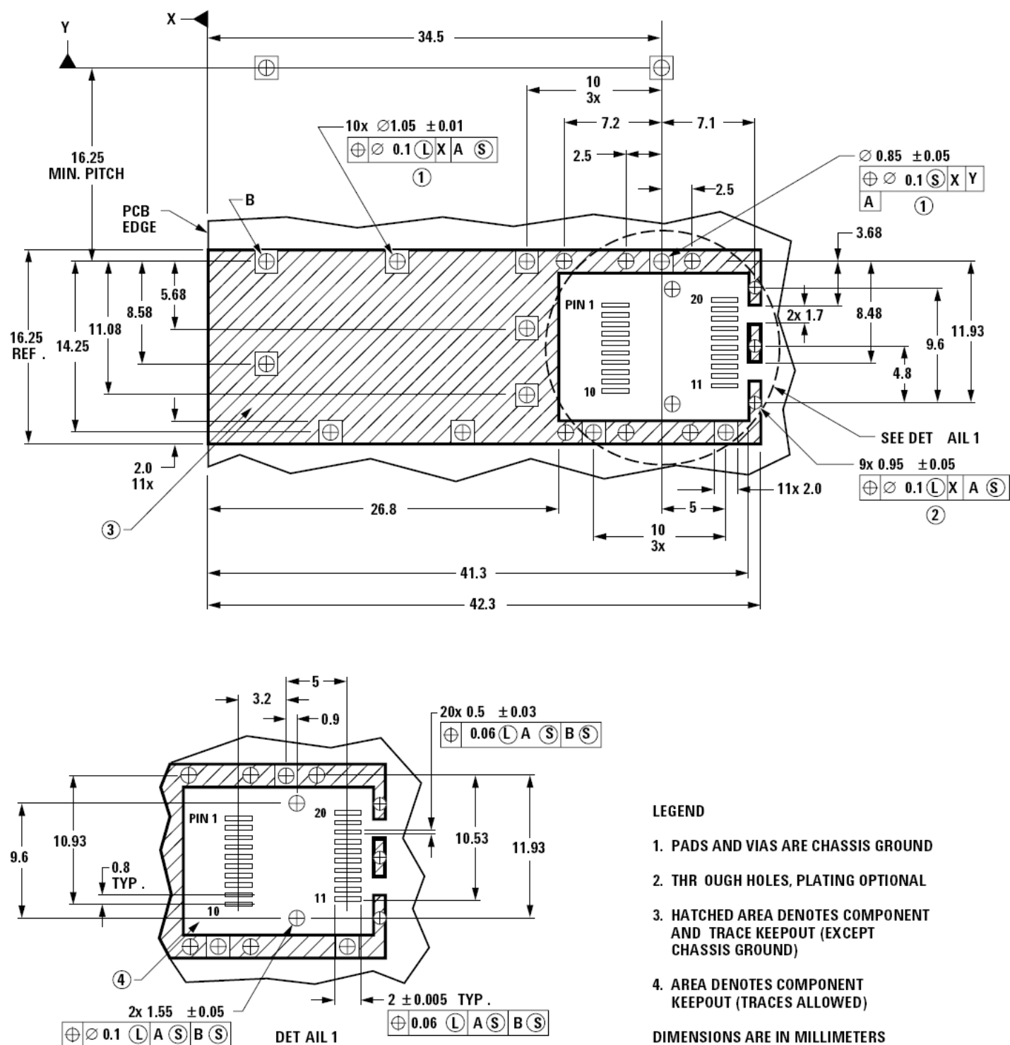
Figure 3: SFP Host Board Mechanical Layout
