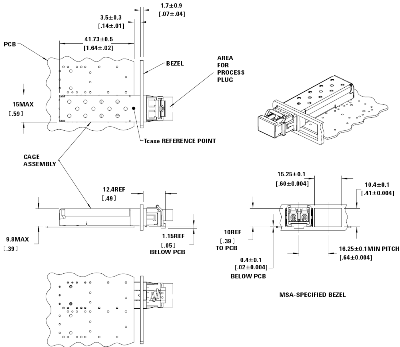
Figure 4: SFP Assemblies Drawing
