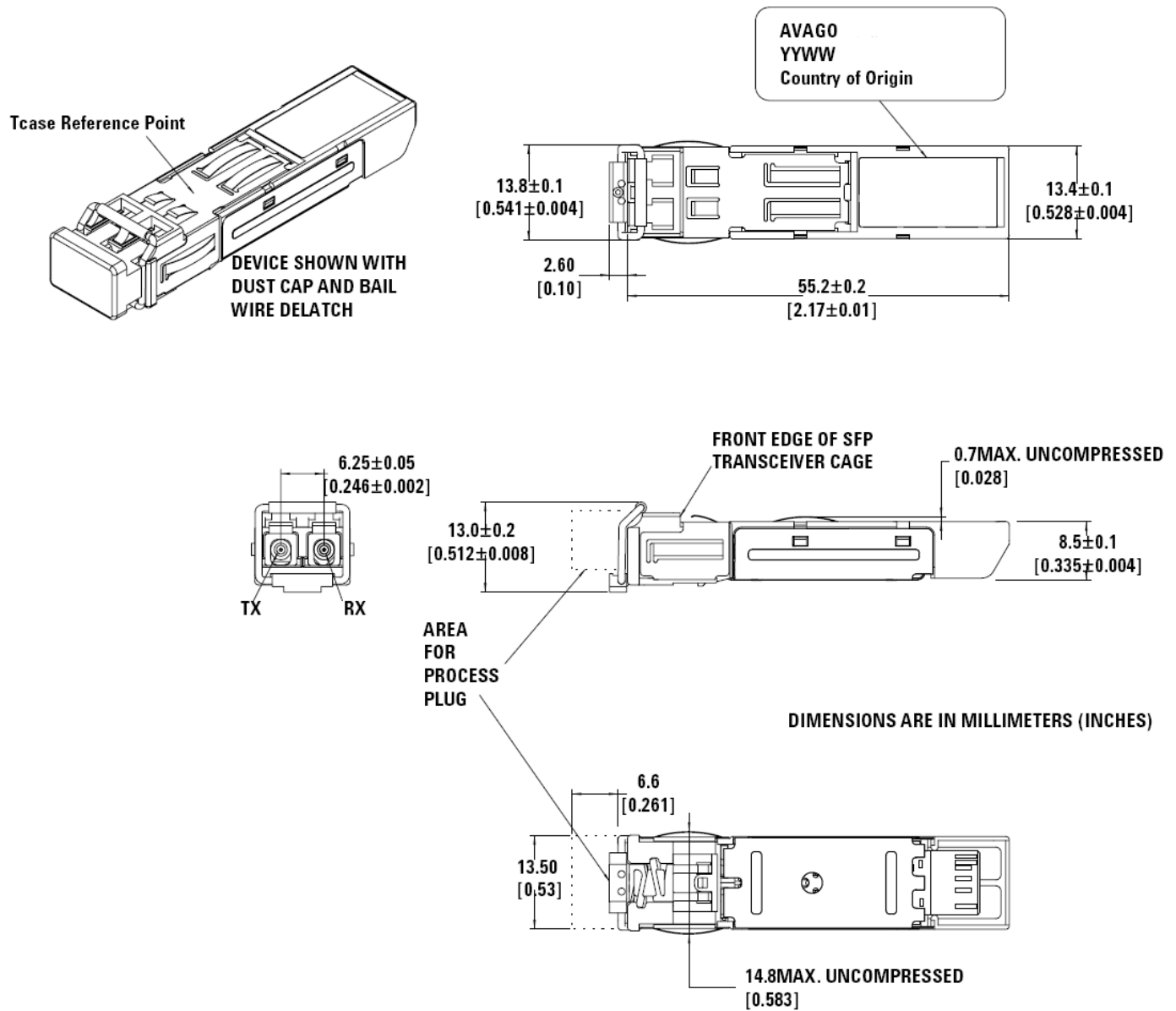
Figure 2: Mechanical Dimensions
