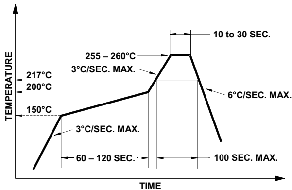
Figure 12: Recommended Lead-Free Reflow Soldering Profile
