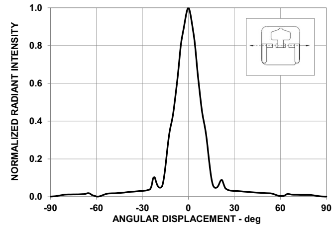
Figure 6: Radiation Pattern: 18°
