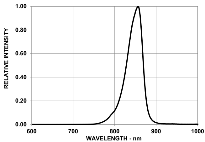
Figure 5: Spectral Distribution
