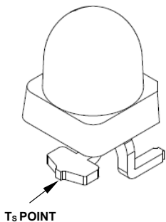
Figure 14: Solder Point Temperature on PCB
