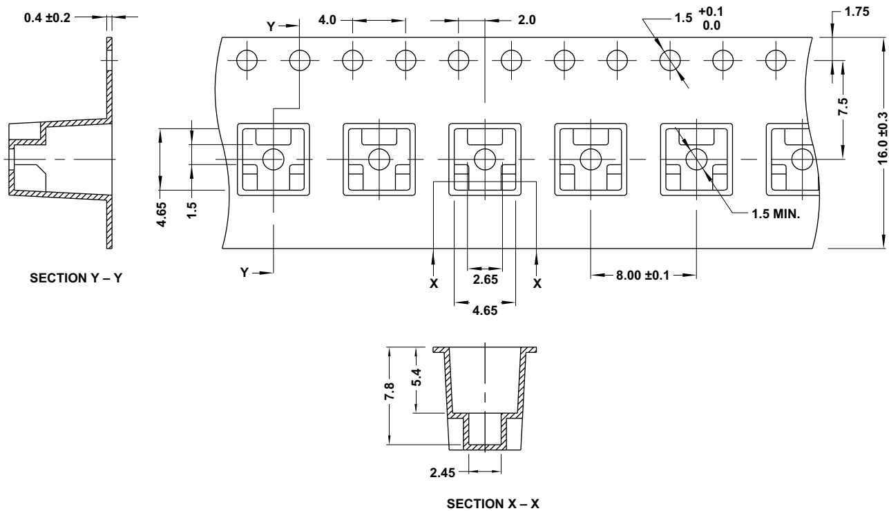
Figure 10: Carrier Tape Dimensions
