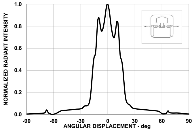
Figure 7: Radiation Pattern: 30°
