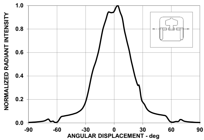
Figure 8: Radiation Pattern: 40°
