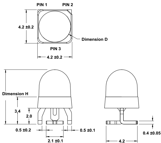
Figure 1: Package Drawing
