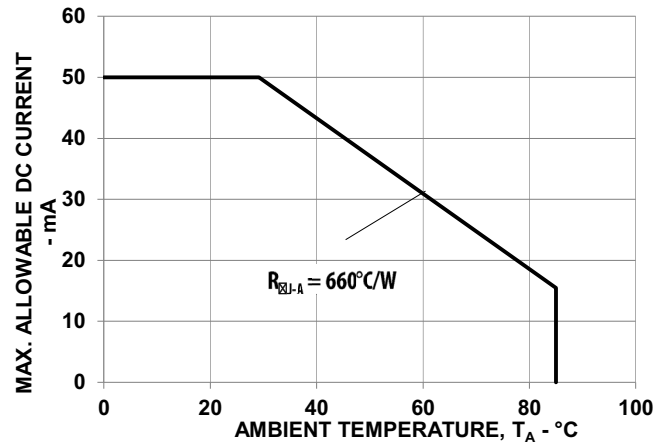
Figure 9: Maximum Forward Current vs. Ambient Temperature. Derate based on T_{J\ MAX} = 110^{\circ}\text{C} .
