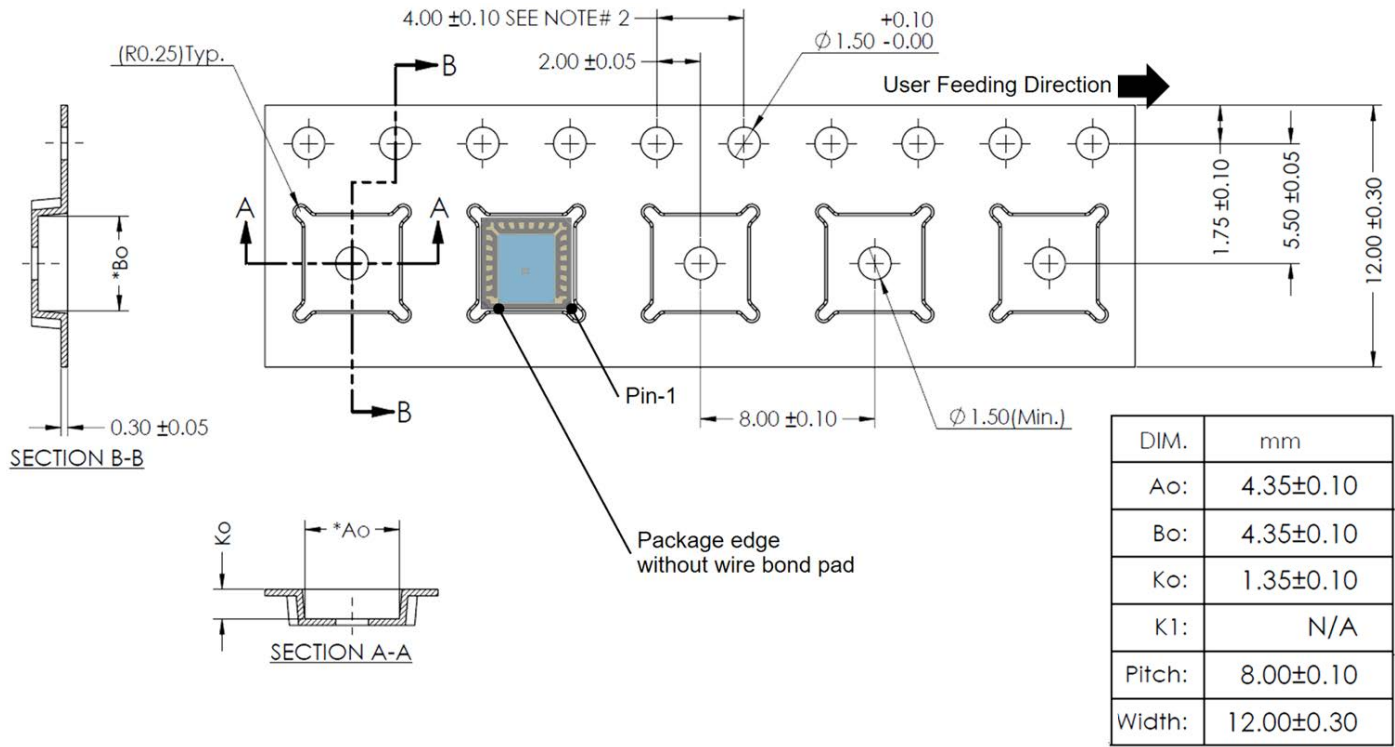
Figure 17: Tape and Reel Feeding Direction
