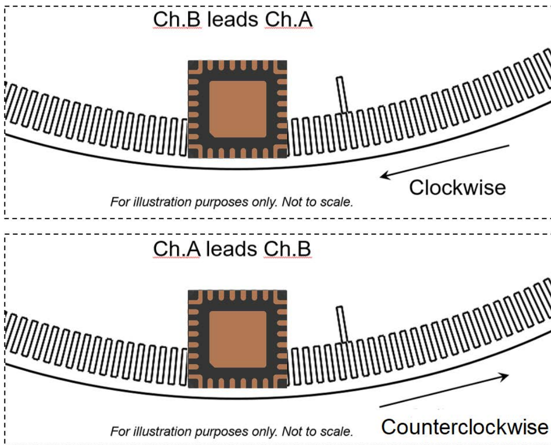
Figure 15: Channel A and Channel B Signal Output Sequence Is with Respect to Code Wheel Rotational Direction
