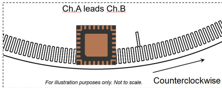
Figure 2: Top View: Code Wheel Movement Direction versus Output Signals
