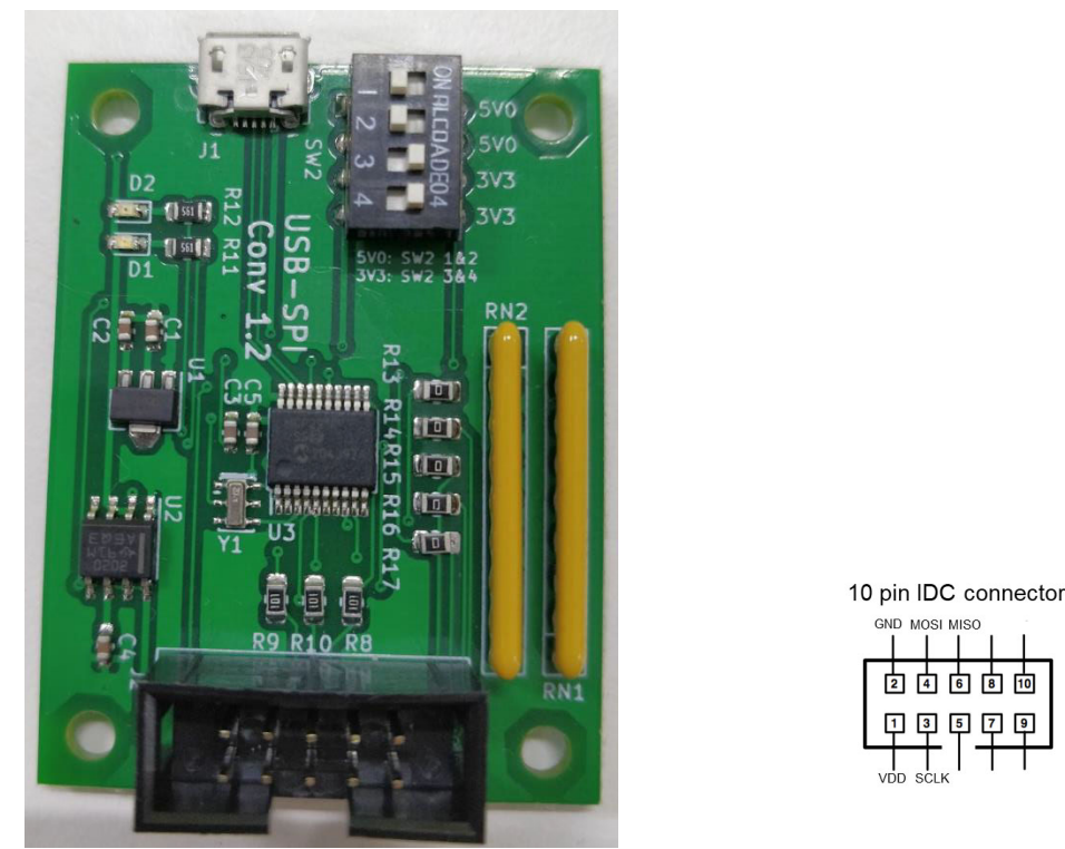
Figure 14: HEDS-9930(E/EL)EVB Evaluation Board
