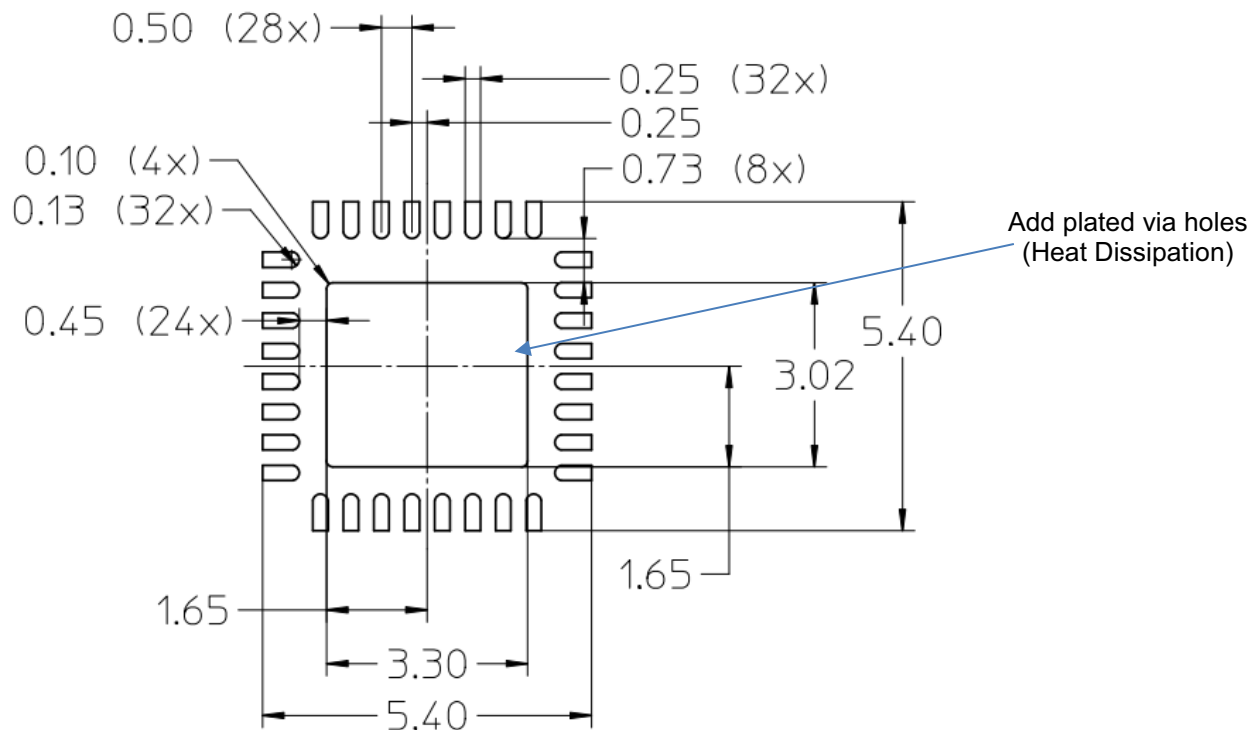
Figure 2: AEDR-9930E/EL PCB Land Pattern
