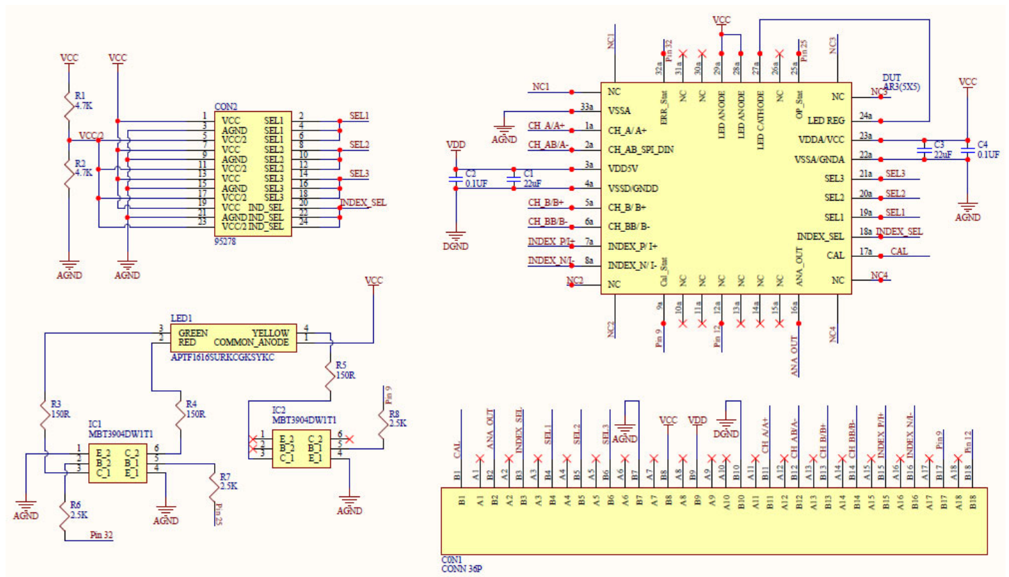
Figure 1: Schematic Diagram for HEDS-9930(E/EL)EVB Evaluation Board
