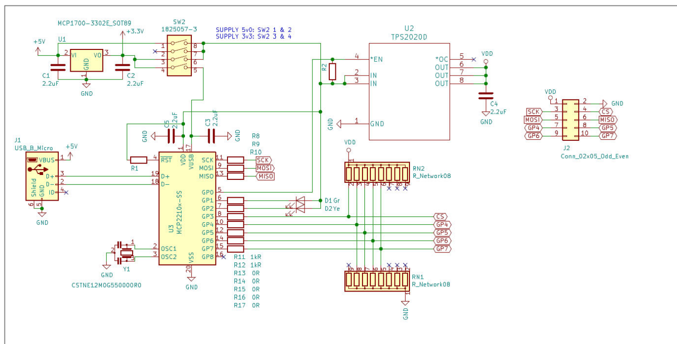
Figure 15: Reference Design for Calibration HEDS-9930(E/EL)PRGEVB Schematic and IDC 10 Pin Assignment
