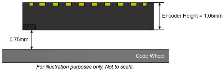
Figure 8: Top Down View of AEDR-9930E with Respect to Code Wheel Positioning
