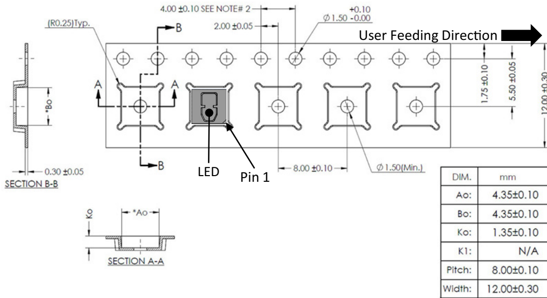
Figure 11: Tape and Reel
