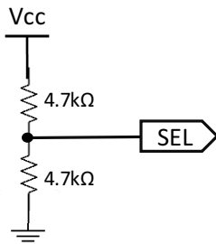
Figure 4: Example of Voltage Divider Circuit
