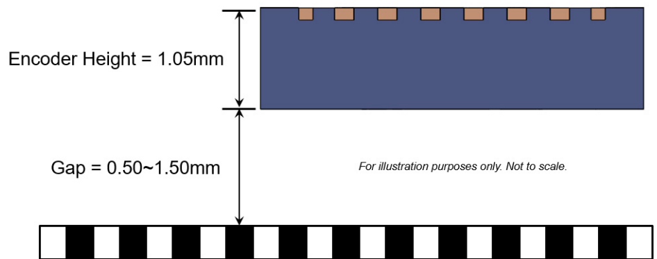
Figure 8: Encoder Placement Orientation
