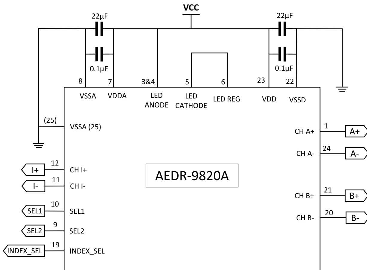
Figure 5: Reference Schematic Diagram for AEDR-9820A
