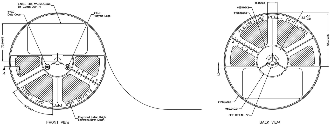
Figure 12: Reel Dimensions
