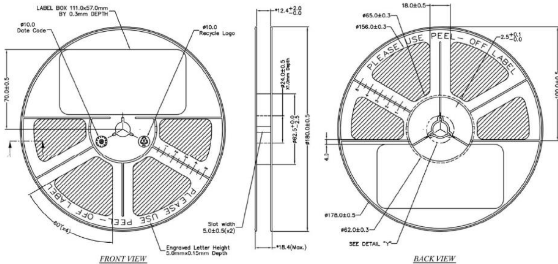
Figure 8: Reel Dimensions
