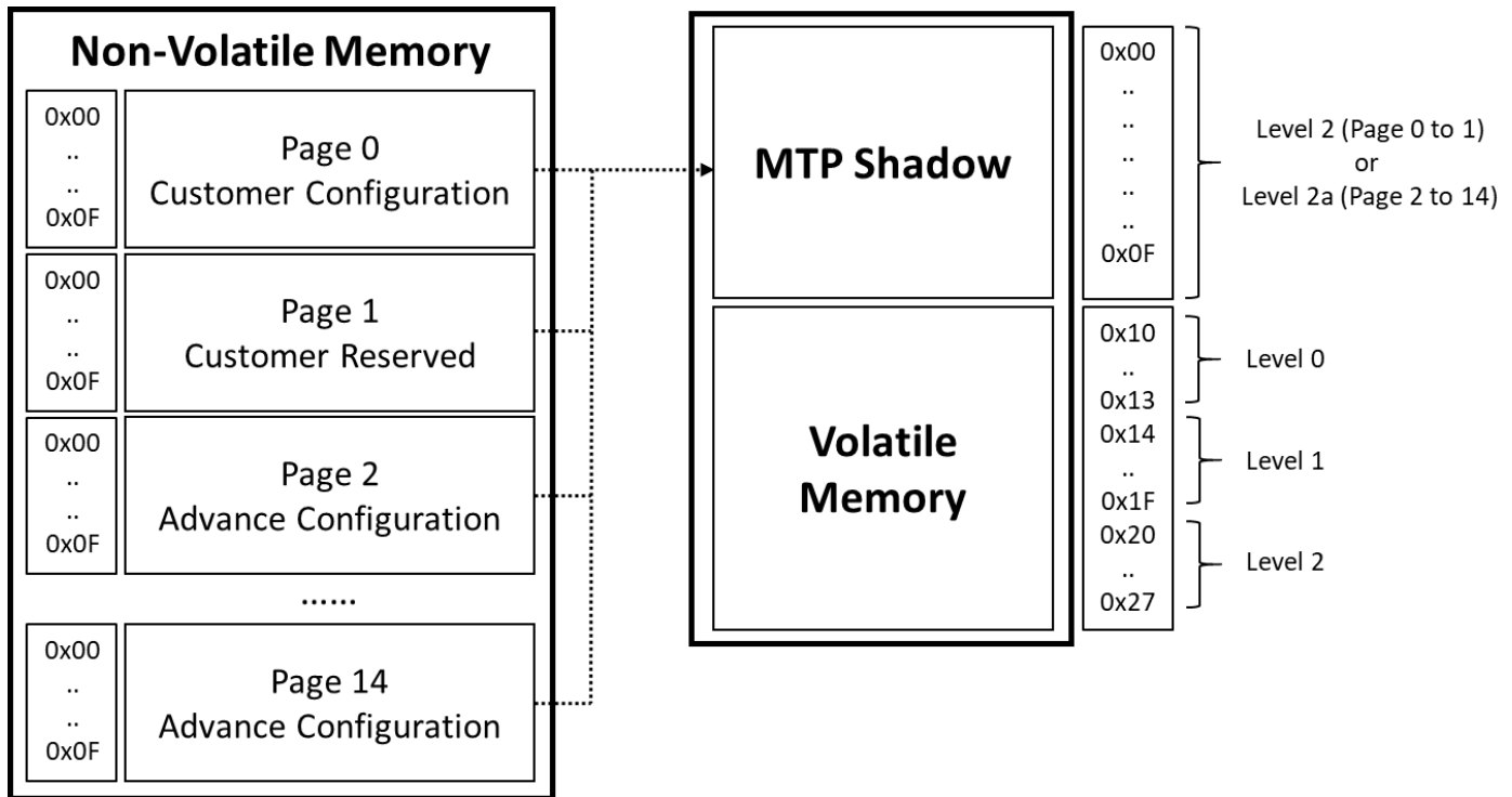
Figure 4: Non-volatile/Volatile Memory and MTP Shadow Block Diagram
