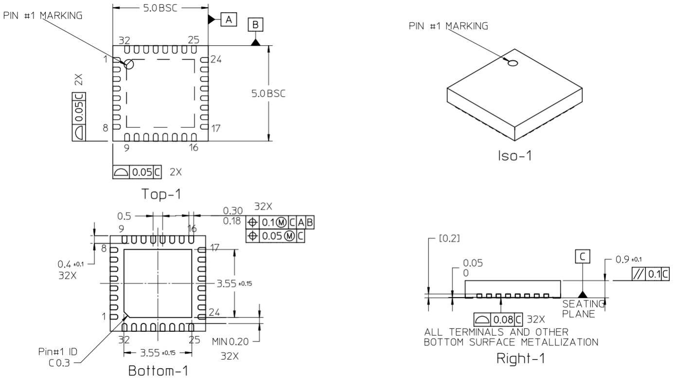
Figure 7: AEAT-9955, 32 QFN Dimensions
