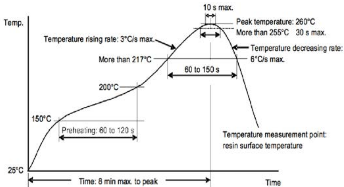
Figure 31: Recommended Lead-Free Solder Reflow Soldering Temperature Profile
