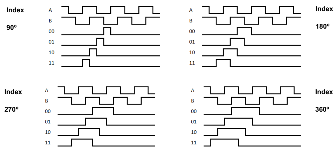
Figure 26: Index Signal Configuration
