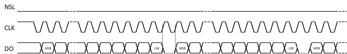
Figure 21: SSI-2(B)
