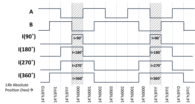
Figure 25: ABI Signal (4096 CPR with Different I-Width Settings)
