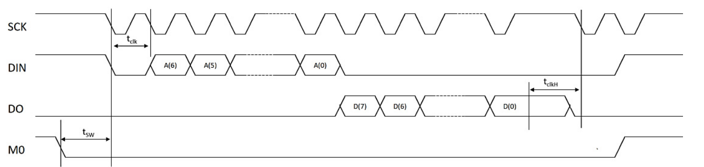
Figure 13: SPI3 Timing Diagram
