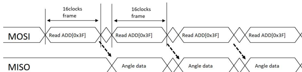
Figure 11: Read Command
