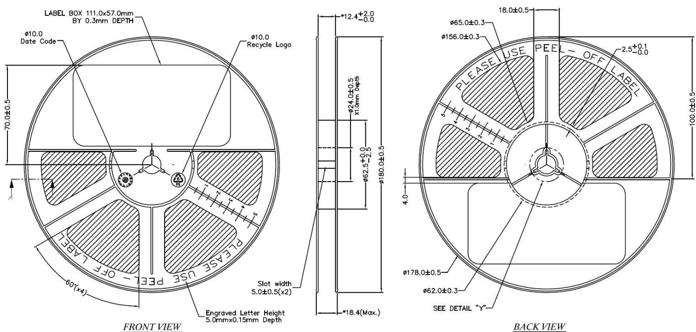
Figure 32: Reel Dimensions
