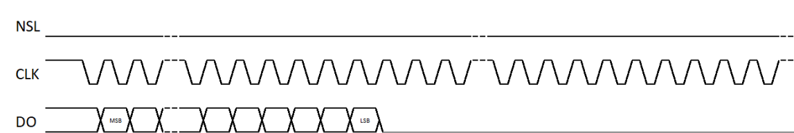
Figure 20: SSI-2(A)
