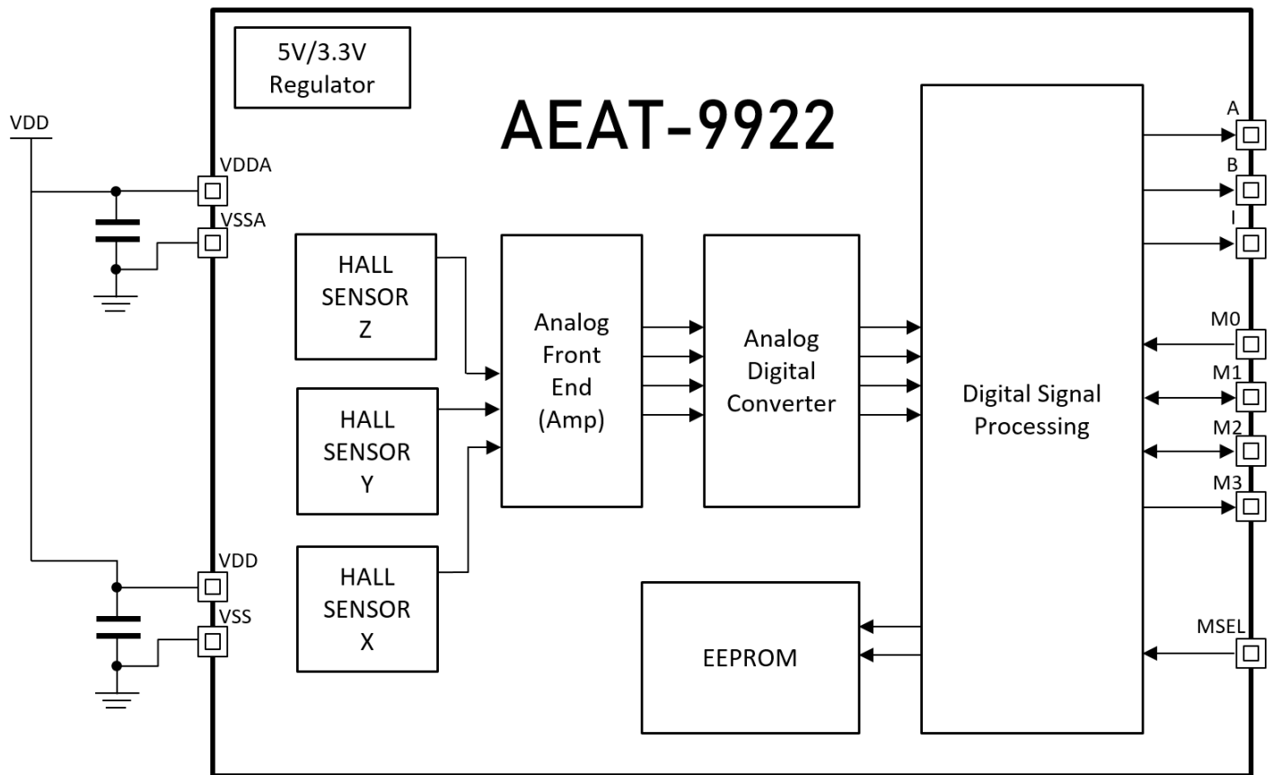
Figure 1: AEAT-9922 Block Diagram
