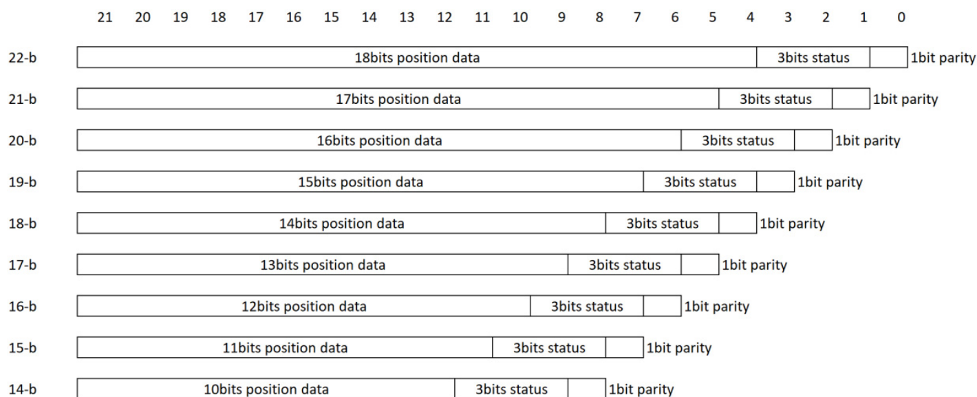
Figure 22: SSI2 Read Data Format
