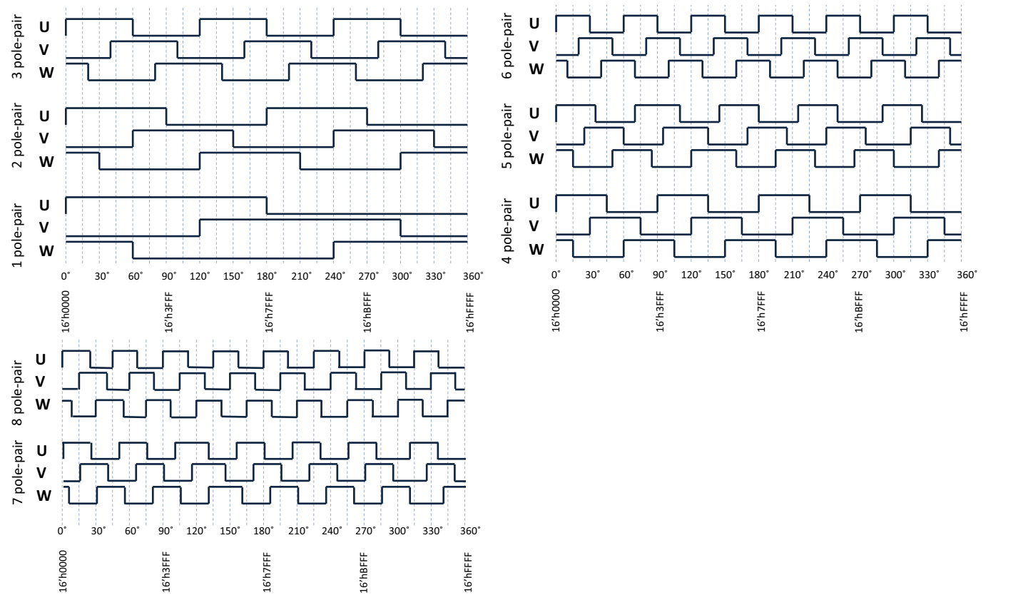
Figure 27: Commutation Output
