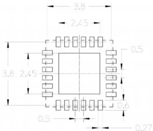
Figure 30: Land Pattern Dimensions
