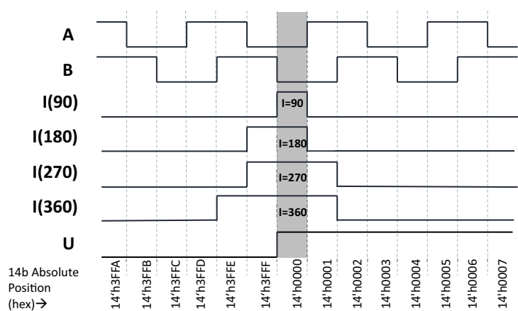
Figure 28: U-to-I Tagging
