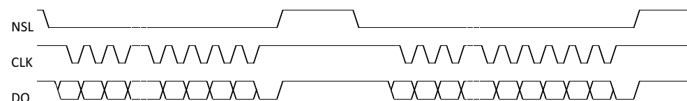
Figure 17: SSI-3(A)
