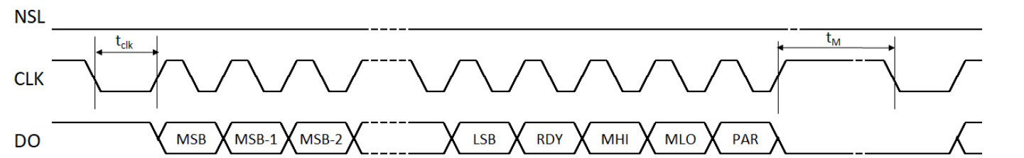
Figure 19: SSI 2-Wire Timing Diagram
