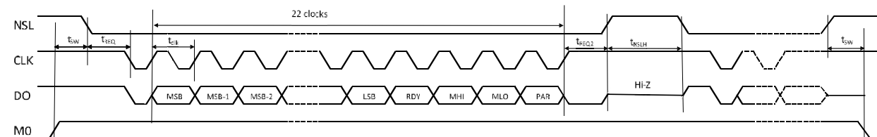
Figure 18: SSI-3(B)
