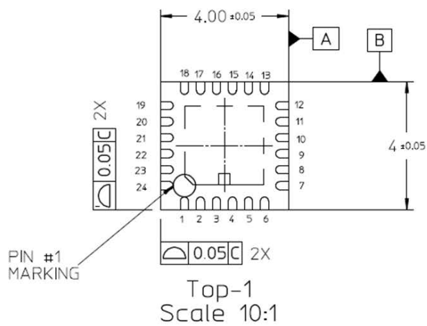
Figure 29: AEAT-9922, 24 QFN Dimensions
