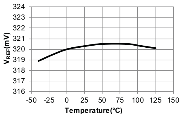
Figure 6: V_{REF} Change vs. Temperature
