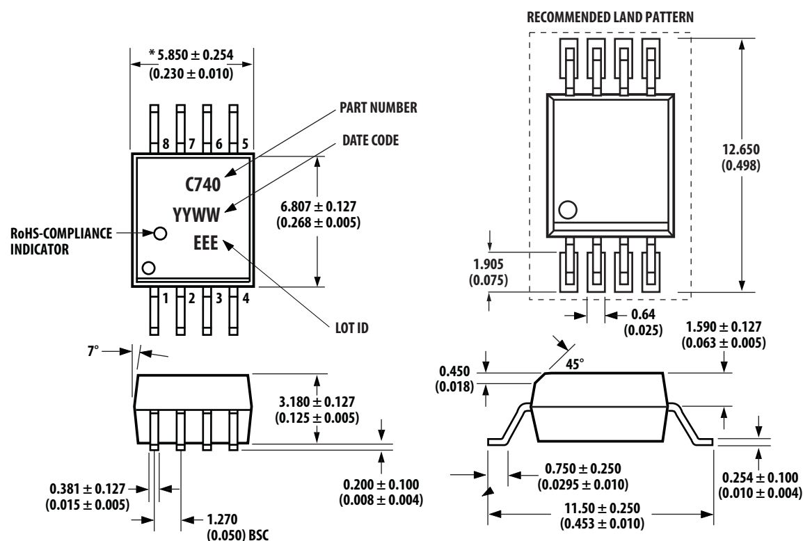
Figure 3: Package Dimensions
