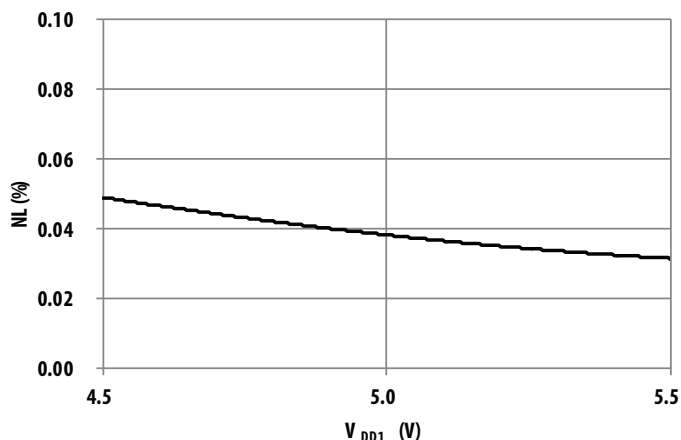
Figure 9: Nonlinearity vs. Supply V_{DD1}
