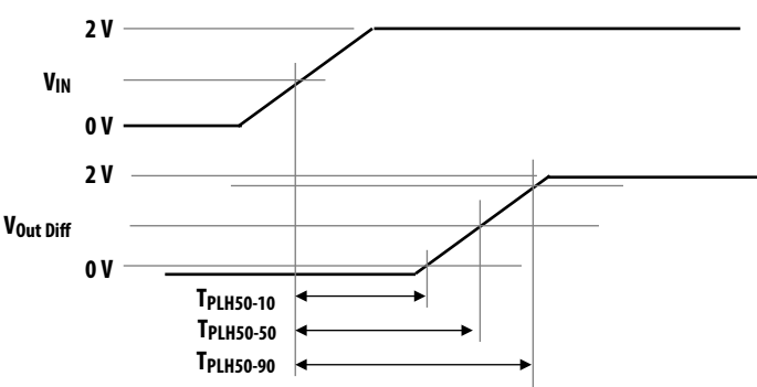
Figure 18: Input to Output Propagation Delay Timing Diagram. V_{Out\ Diff} = V_{Out+} - V_{Out-}
