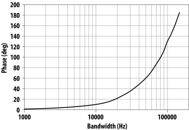
Figure 15: Phase Response
