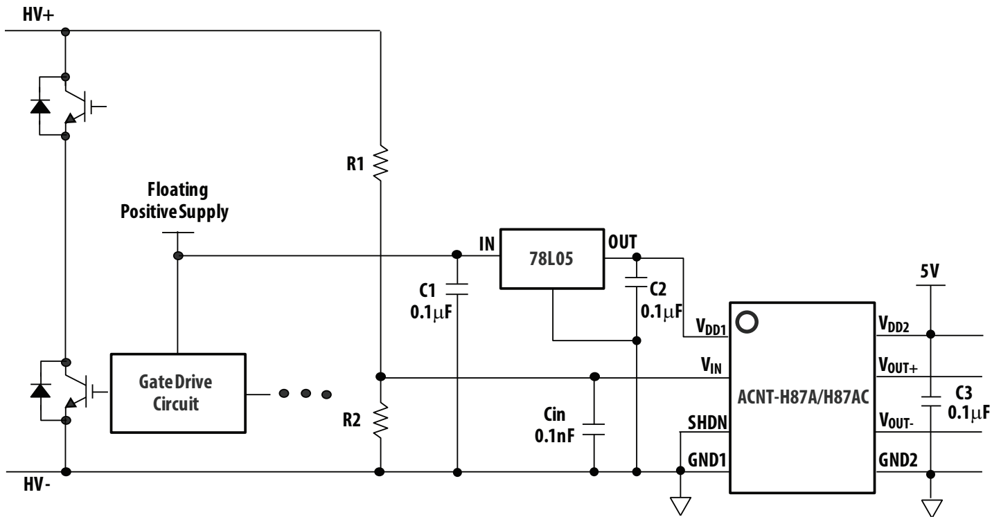
Figure 22: Recommended Power Supply and Bypassing
