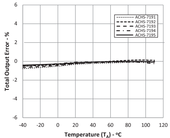
Figure 4: Total Output Error @ I P(MAX) vs. Temperature
