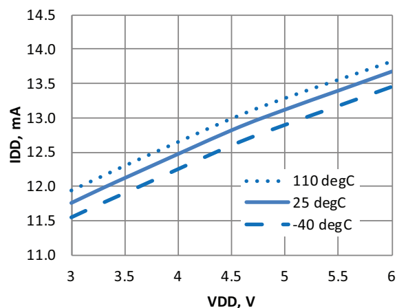
図8 : Supply Current vs. Supply Voltage
