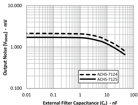
図5 : Output Noise vs. External Filter Capacitance
