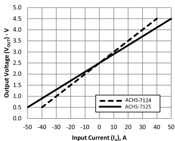
図4 : Output Voltage vs. Input Current
