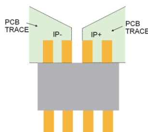
図13： Recommended Trace Layout on the Input Pins
