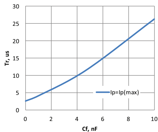
図10 : Rise Time vs. External Filter
