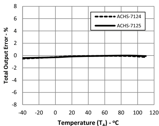
図6 : Total Output Error at I_{P(MAX)} vs. Temperature
