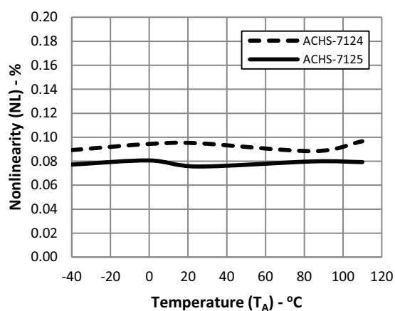
図3 : Nonlinearity vs. Temperature
