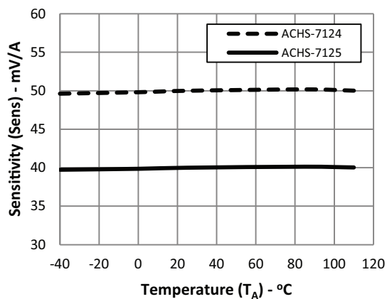
図1 : Sensitivity vs. Temperature
