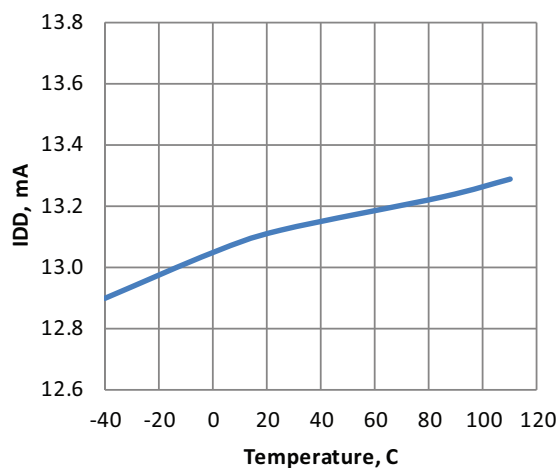
図7 : Mean Supply Current vs. Temperature
