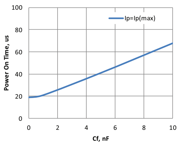
図9 : Power-on Time vs. External Filter
