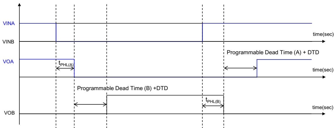
Figure 32: Timing Diagram with Programmable Dead Time
