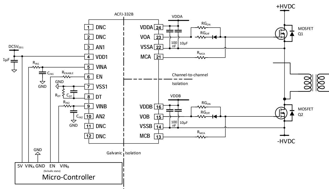
Figure 30: ACFJ-332B Typical Application Circuit
