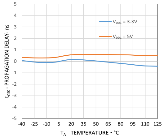
Figure 15: Channel-to-Channel Skew vs Temperature
