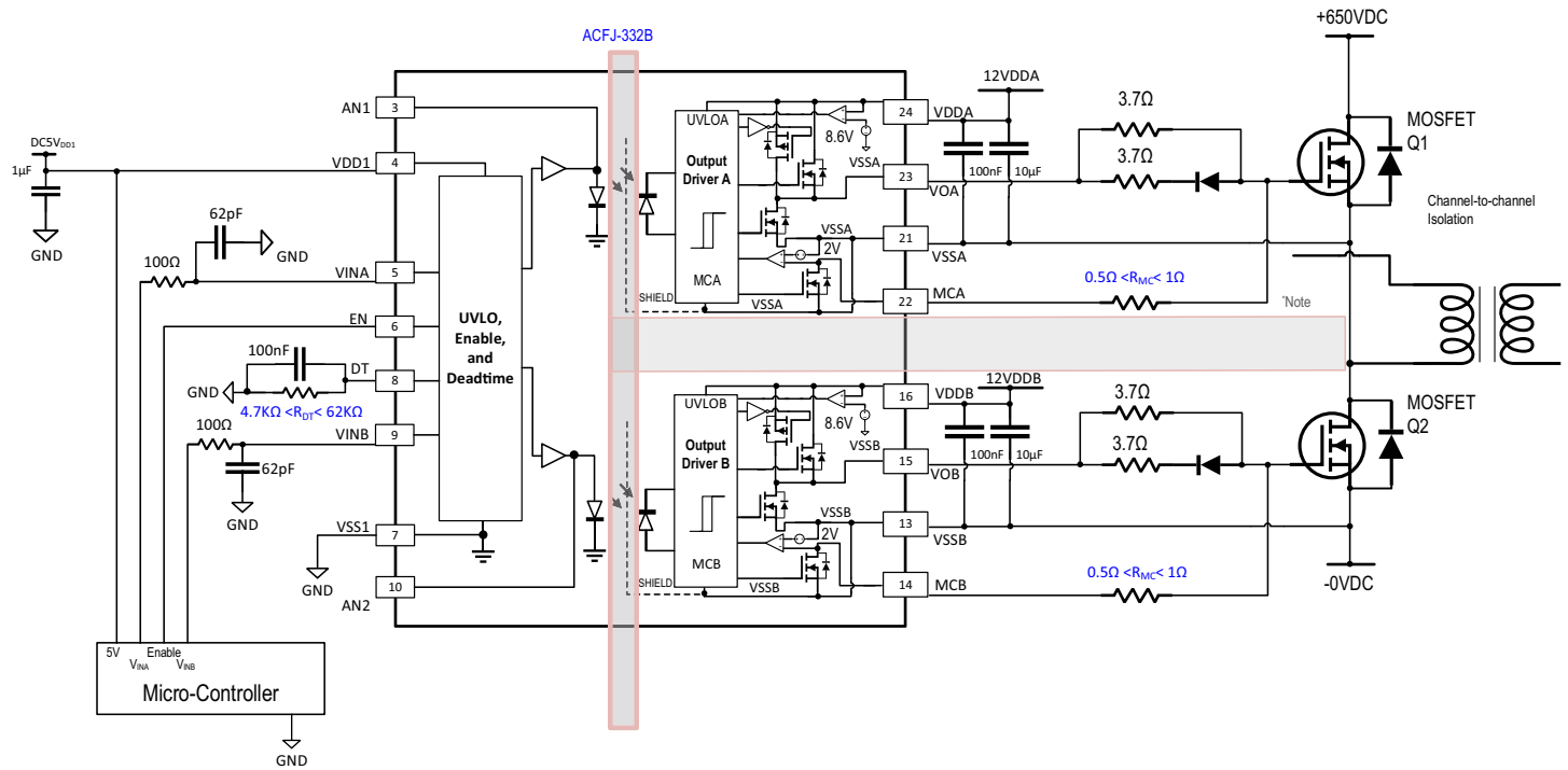
Figure 31: Example ACFJ-332B Gate Driver Circuit with Silicon MOSFET Application Circuit Diagram
