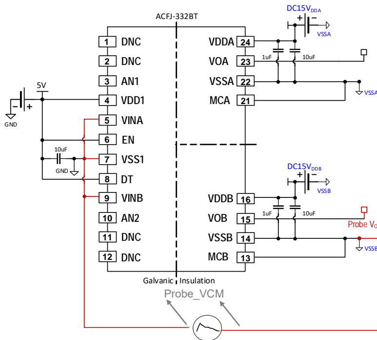
Figure 8: CMR V_O Low Test Circuit
