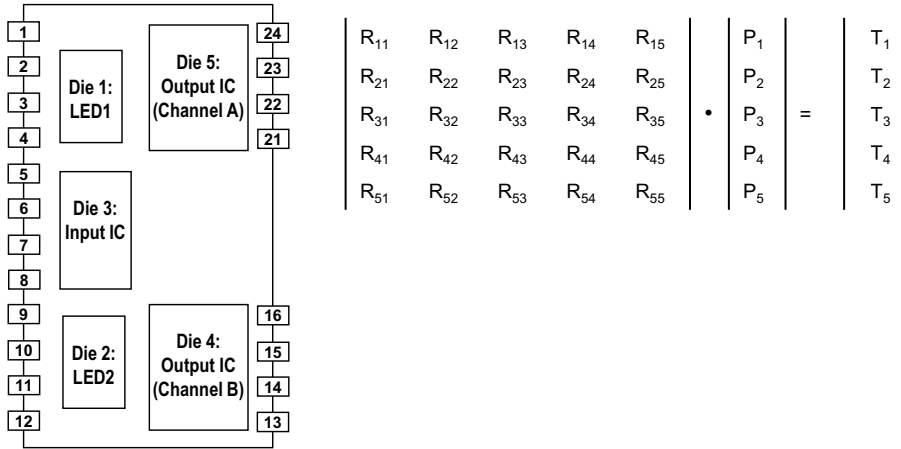
Figure 9: Diagram of ACFJ-332B for Thermal Resistance Model
