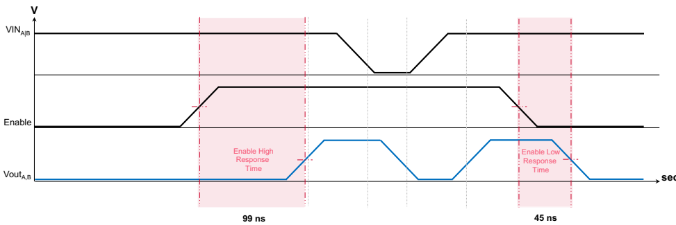
Figure 33: Enable Response Time
