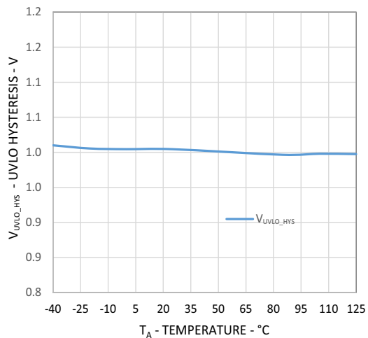
Figure 17: UVLO_{A,B} Hysteresis vs Temperature
