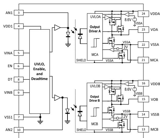
Figure 1: ACFJ-332B Functional Diagram
