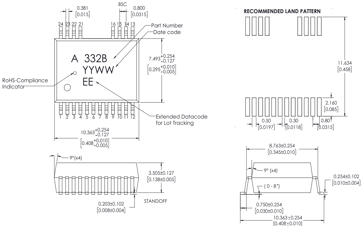
Figure 2: ACFJ-332B Package Outline Drawing
