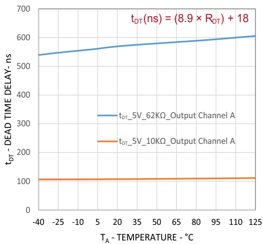
Figure 28: Channel A Dead Time vs. Temperature
