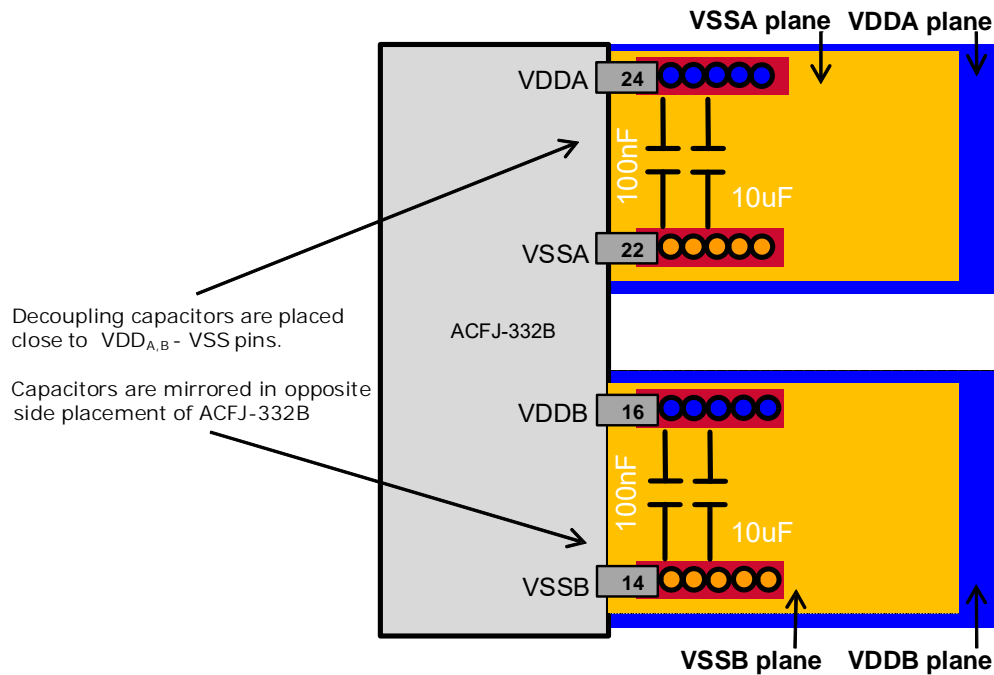
Figure 35: PCB Planes Stack-Up and Bypass Capacitors Placement
