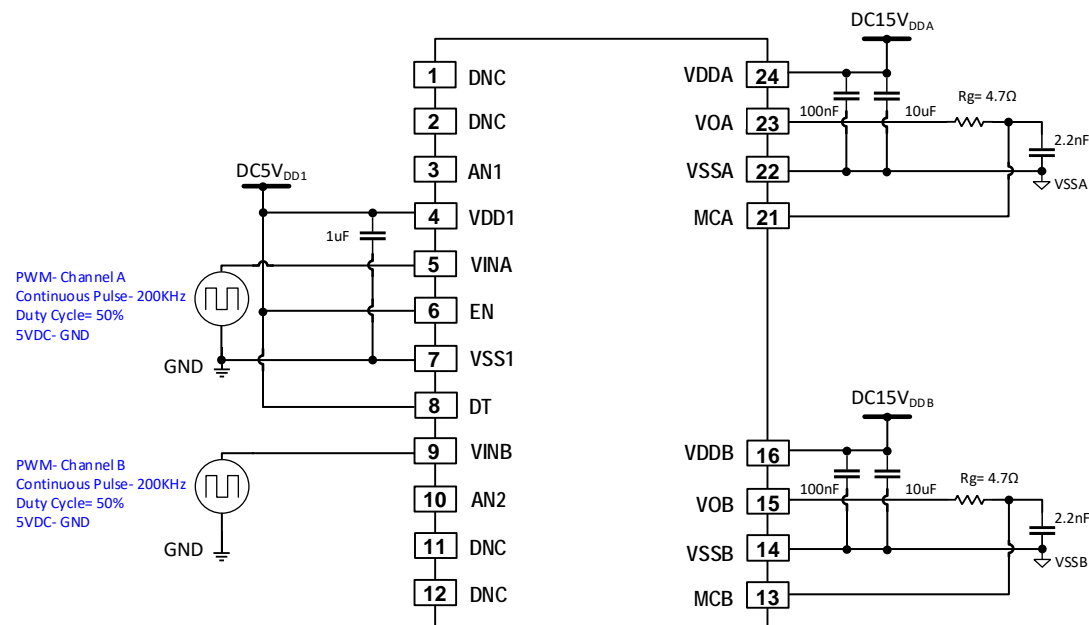
Figure 4: Propagation Delay Measurement Test Setup
