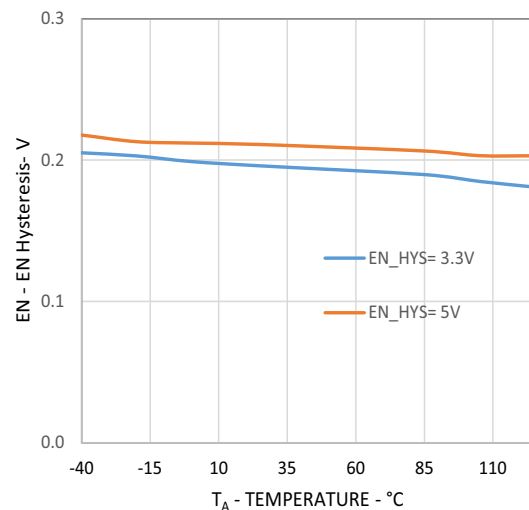
Figure 23: Enable Hysteresis vs Temperature
