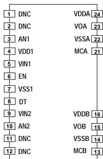
Figure 3: ACFJ-332B Pin Configuration
