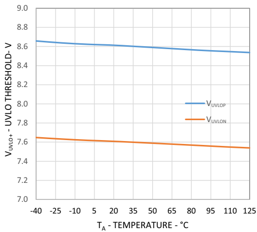
Figure 16: UVLO_{A,B} Threshold vs Temperature
