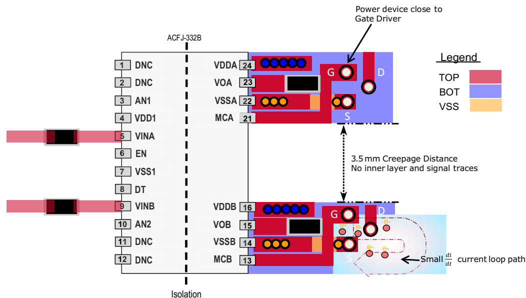
Figure 34: PCB Layout Guidelines
