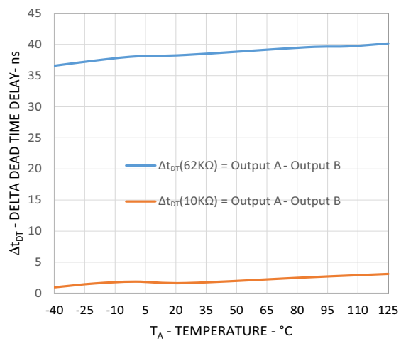
Figure 29: Dead Time Matching vs. Temperature
