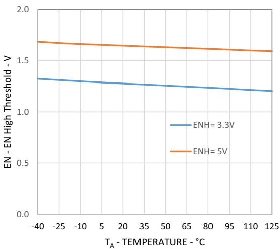
Figure 22: Enable High Threshold vs Temperature
