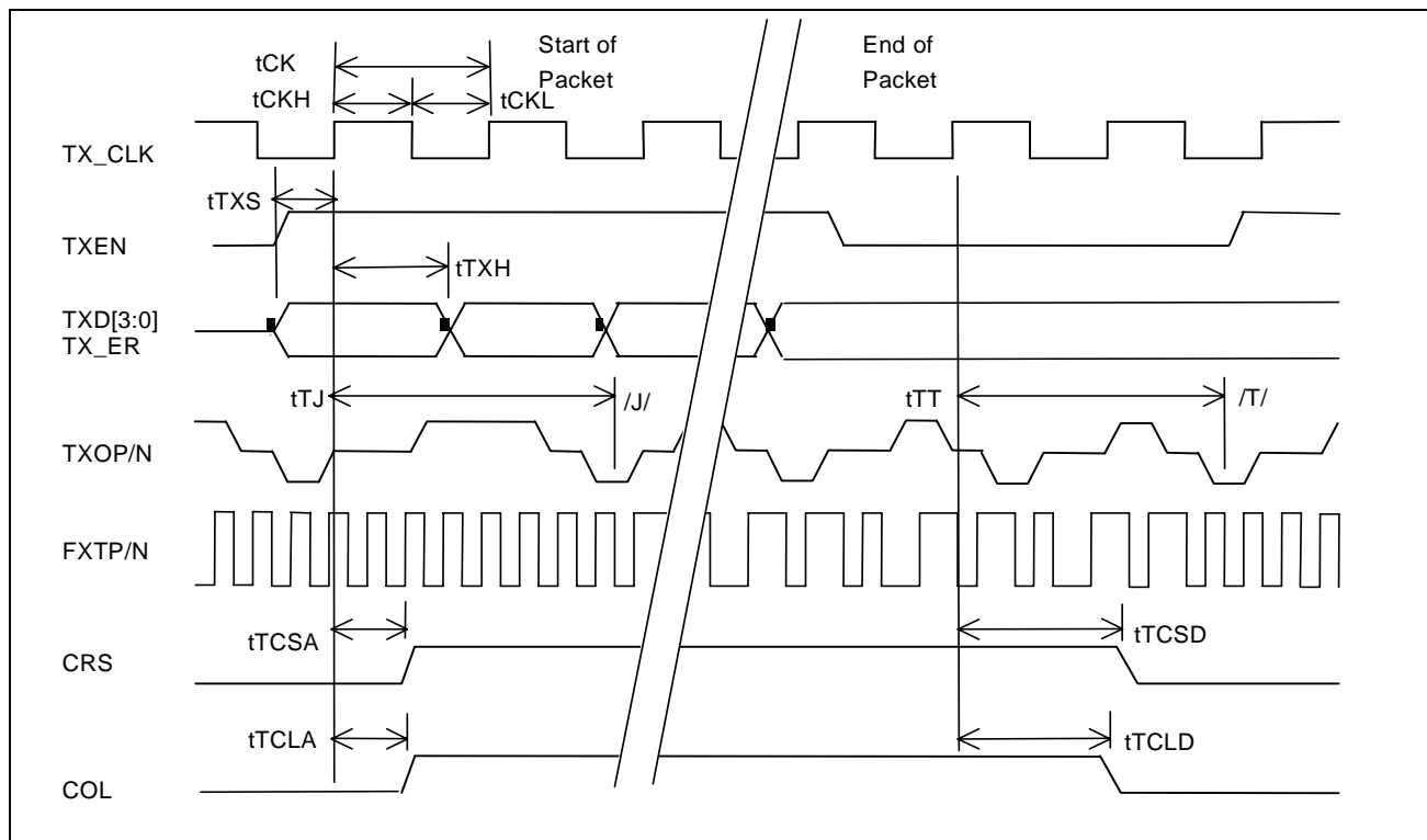
Figure 5: 100BASE-TX/FX MII Transmit Timing
