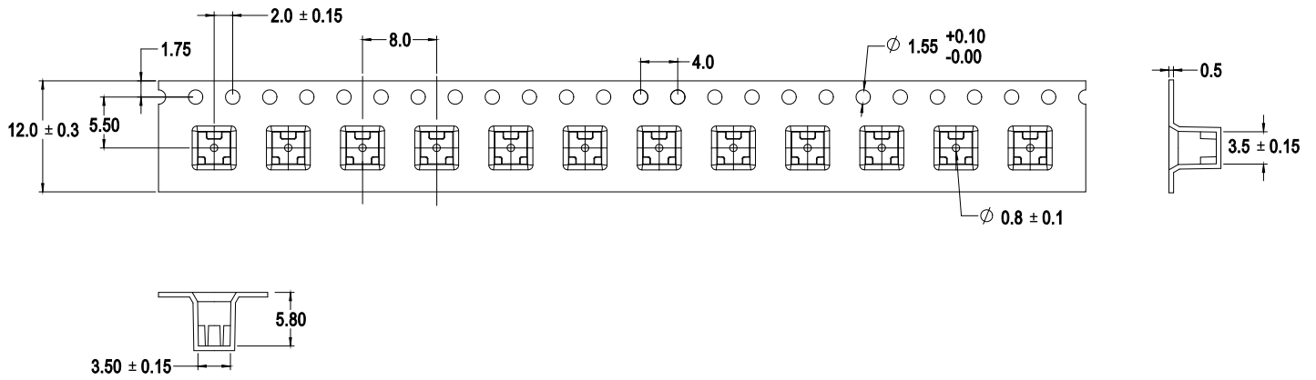
Figure 12: Carrier Tape Dimensions
