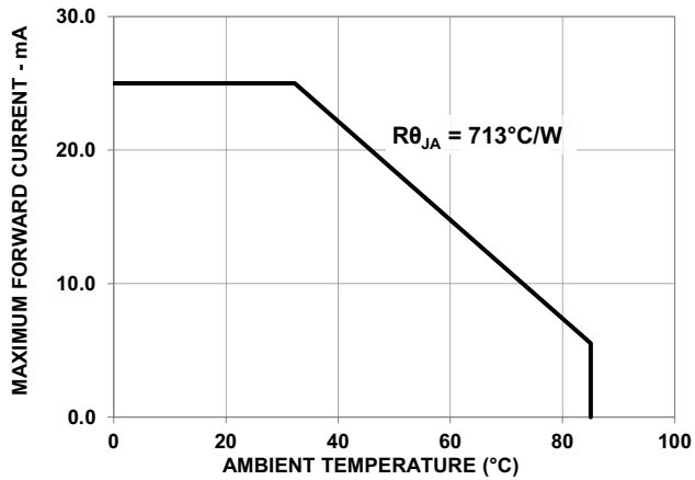
Figure 10: Maximum Forward Current vs. Ambient Temperature. Derate Based on T_{J\ MAX} = 100^\circ\text{C} .
