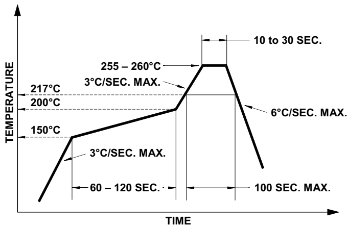
Figure 14: Recommended Lead-Free Reflow Soldering Profile
