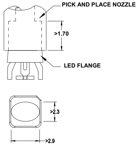
Figure 15: Recommended Nozzle Dimension
