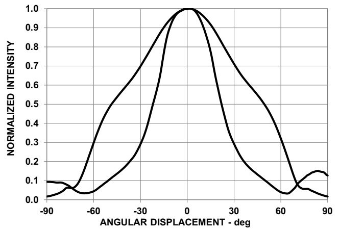
Figure 9: Radiation Pattern
