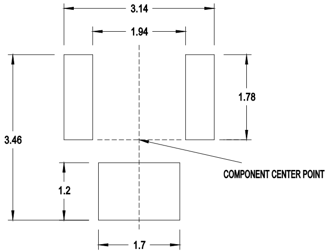
Figure 11: Recommended Soldering Land Pattern
