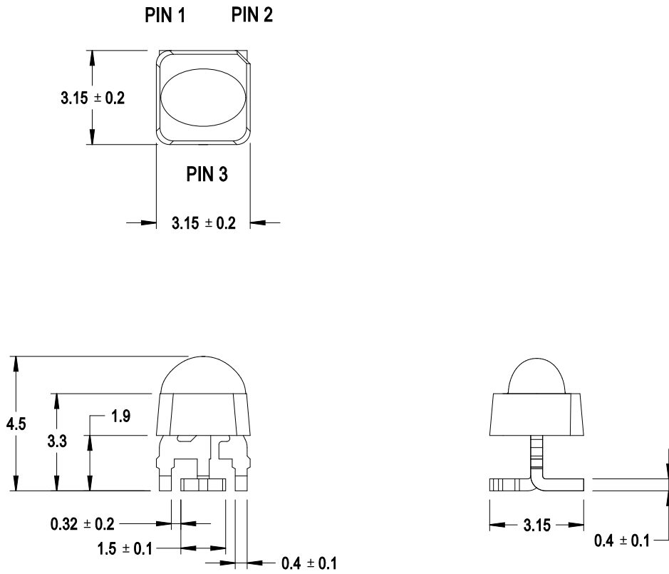
Figure 1: Package Drawing
