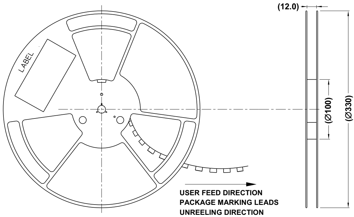
Figure 13: Reel Dimensions
