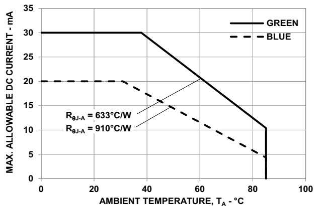
Figure 9: Maximum Forward Current vs. Ambient Temperature. Derate Based on T_{J\ MAX} = 110^\circ\text{C} (Green), T_{J\ MAX} = 100^\circ\text{C} (Blue)
