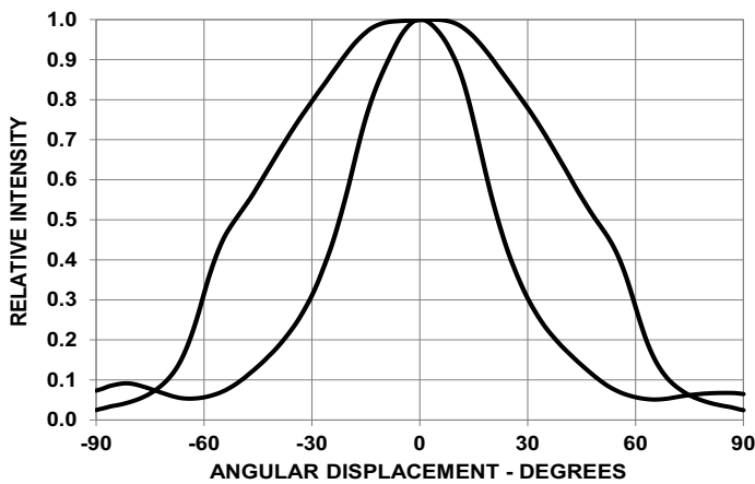
Figure 8: Radiation Pattern
