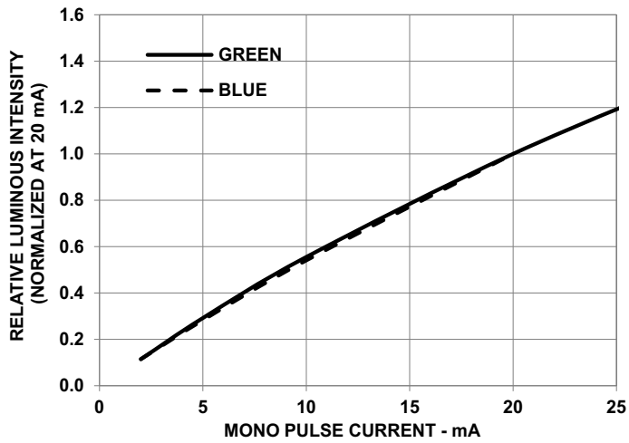
Figure 4: Relative Luminous Intensity vs. Mono Pulse Current
