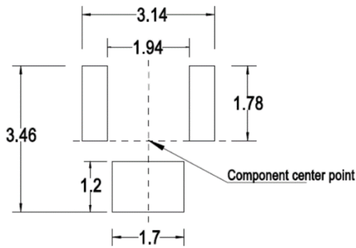
Figure 10: Recommended Soldering Land Pattern
