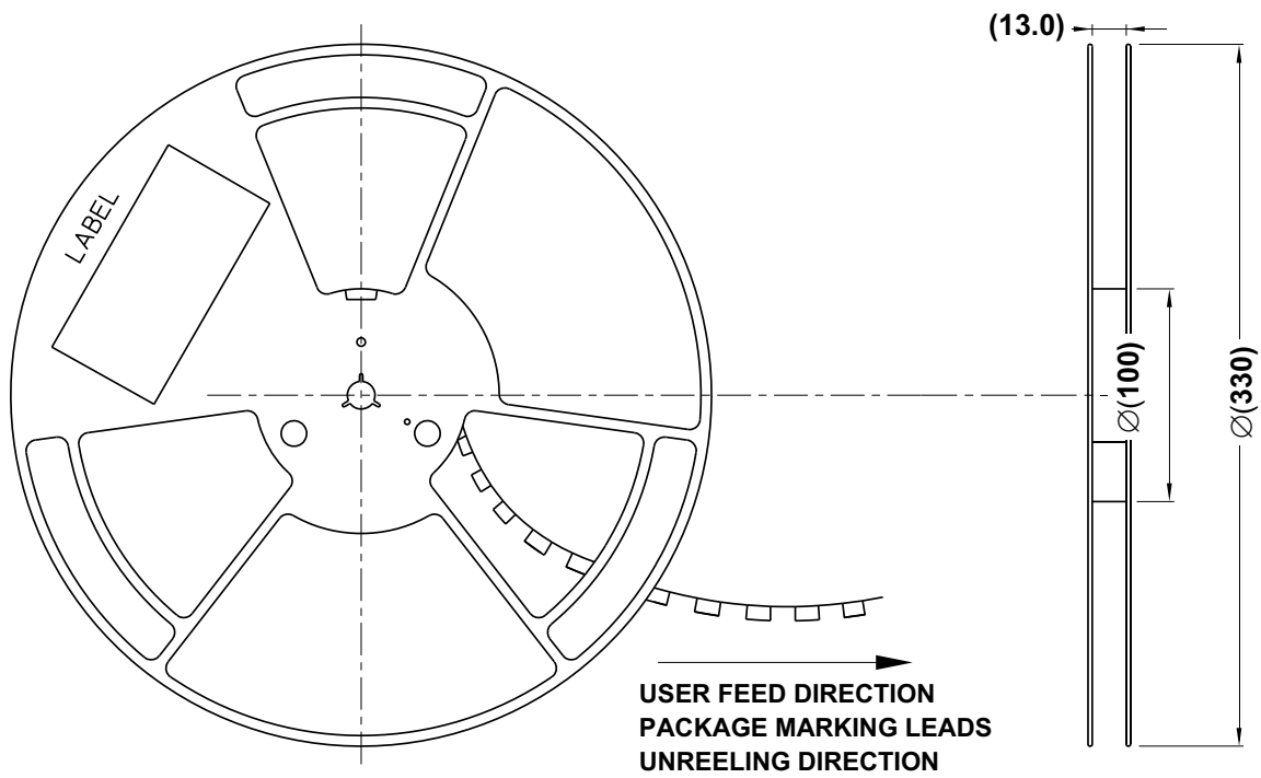
Figure 12: Reel Dimensions
