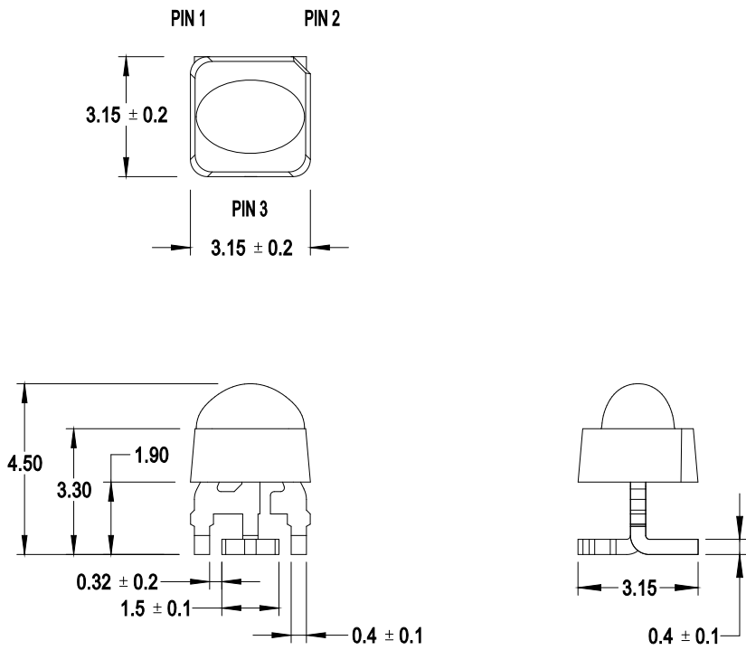
Figure 1: Package Drawing
