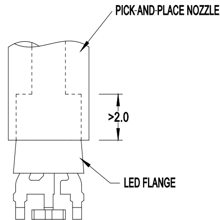
Figure 14: Recommended Nozzle Dimension
