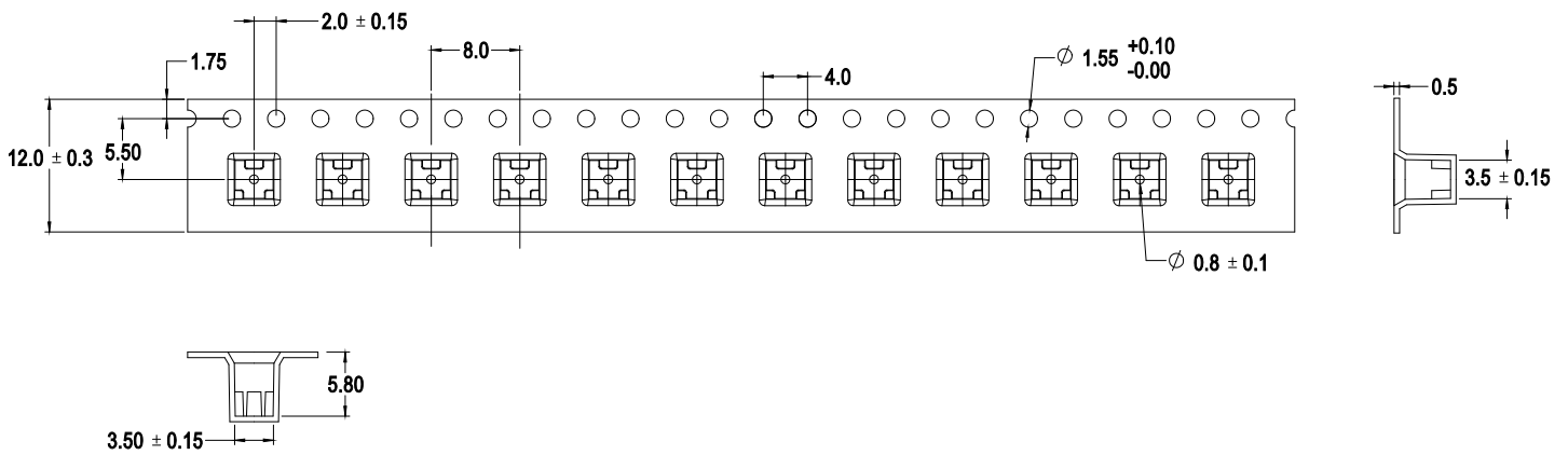
Figure 11: Carrier Tape Dimensions
