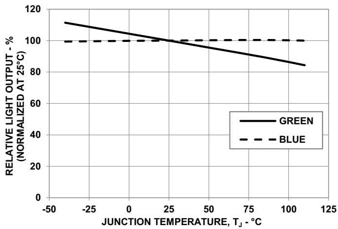
Figure 6: Relative Light Output vs. Junction Temperature
