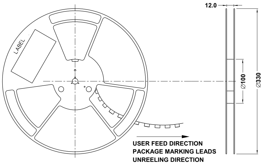
Figure 12: Reel Dimensions
