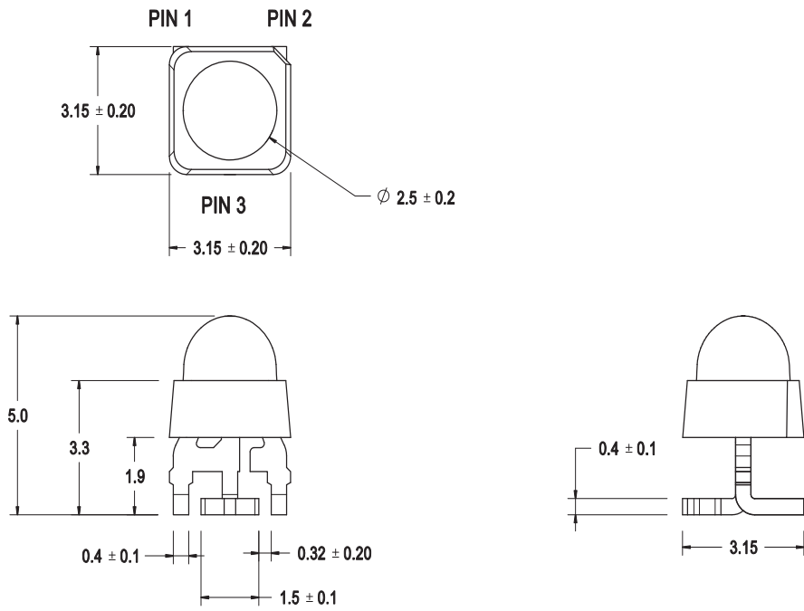
Figure 1: Package Drawing
