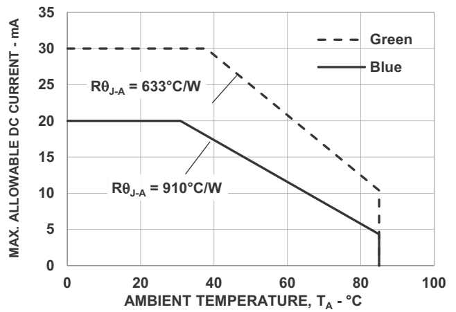
Figure 9: Maximum Forward Current vs. Ambient Temperature. Derate based on T_{J\ MAX} = 110^{\circ}\text{C} (Green), T_{J\ MAX} = 100^{\circ}\text{C} (Blue).
