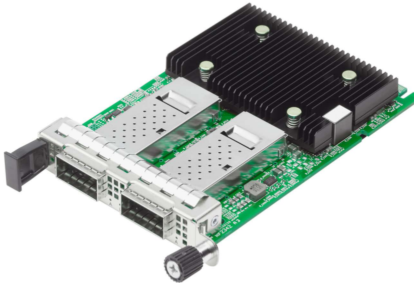
Figure 3: BCM957608-N2200GQP00 Network Interface Controller
