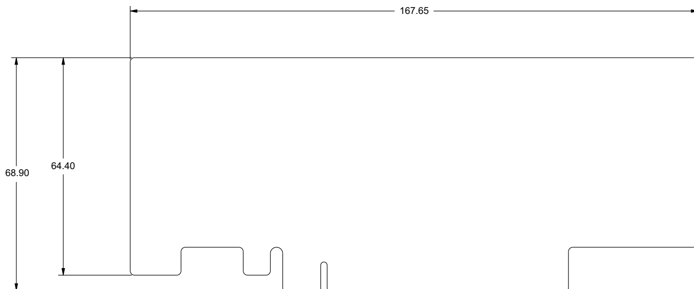
Figure 13: Board Physical Dimensions
