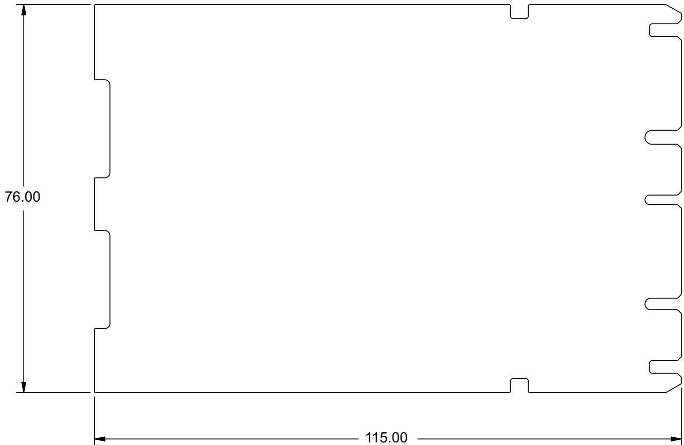
Figure 14: Physical Dimensions (in millimeters)
