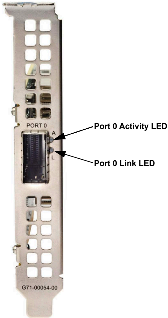
Figure 3: Activity and Link LED Locations
