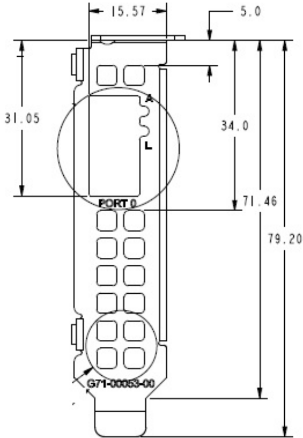
Figure 6: Low-Profile Bracket Outline and Dimensions
