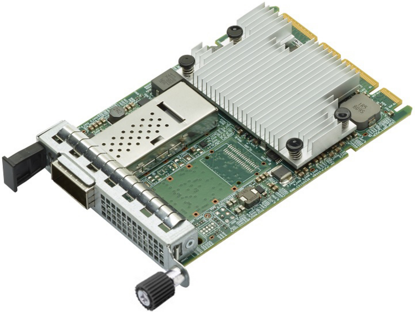
Figure 1: BCM957502-N150G OCP 3.0 SFF Network Adapter
