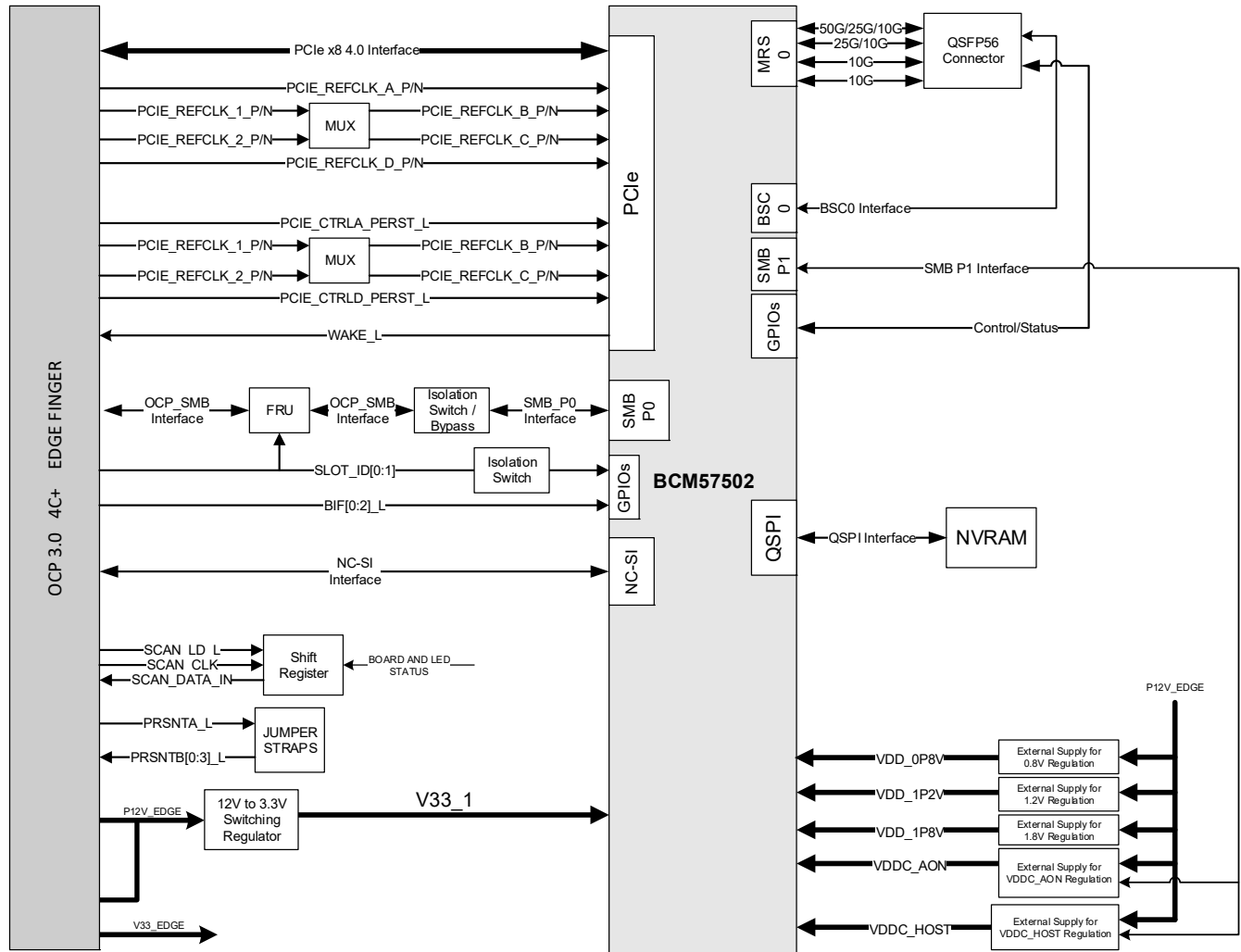
Figure 2: BCM957502-N150G Block Diagram
