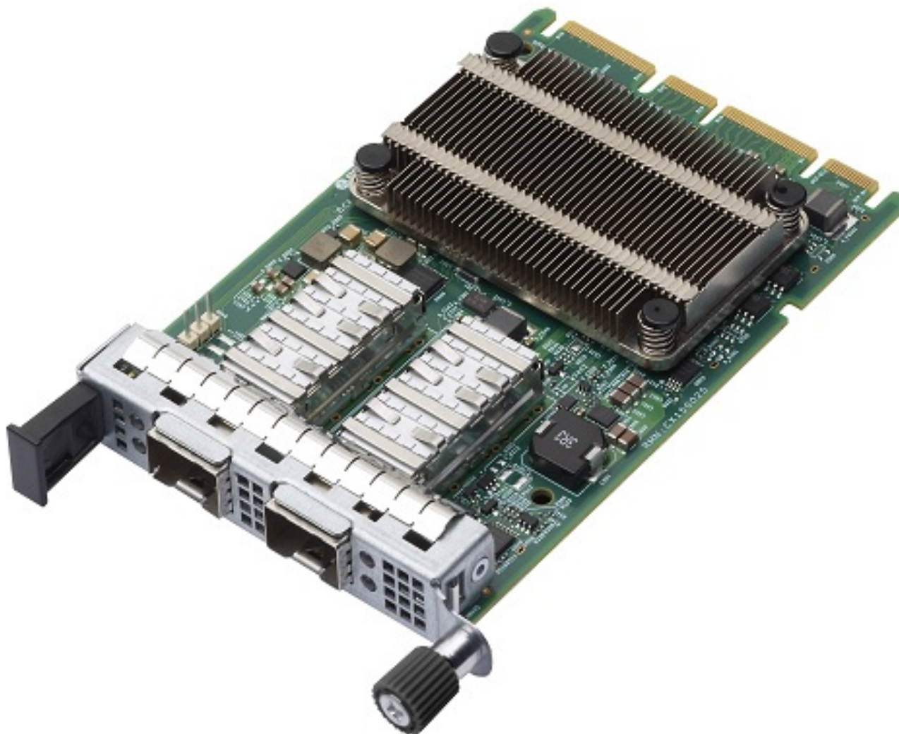
Figure 1: BCM957412N4120C OCP 3.0 SFF Network Adapter
