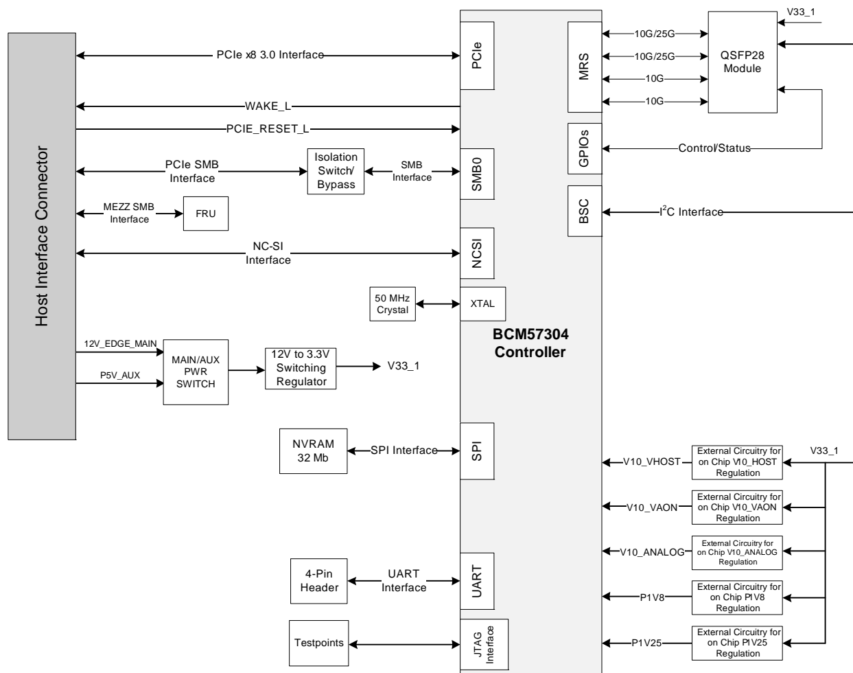
Figure 2: BCM957304M3041C Block Diagram
