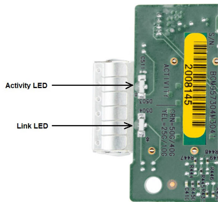
Figure 4: Activity and Link LED Locations
