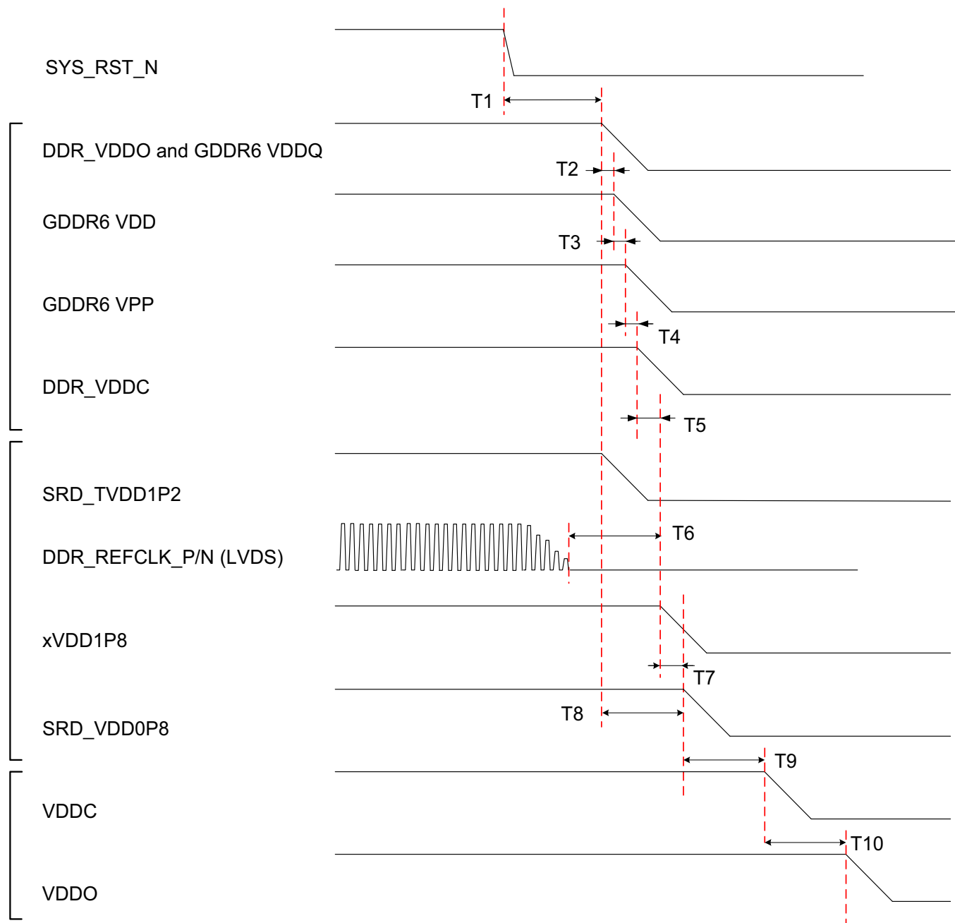
Figure 10: Power-Down Sequence
