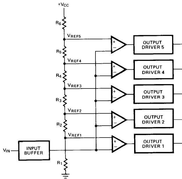
Figure 3. Typical Analog Input Bar Graph Decoder
