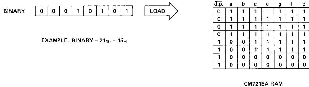
Figure 13. Subroutine LOAD
