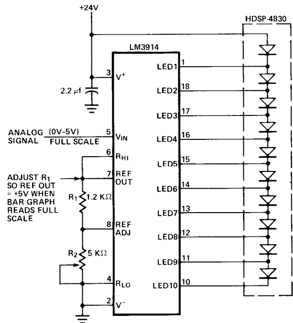
Figure 6. Low Power 0 V - 5 V Bar Graph Meter
