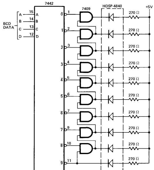
Figure 8. BCD to 10-Element Bar Graph Array
