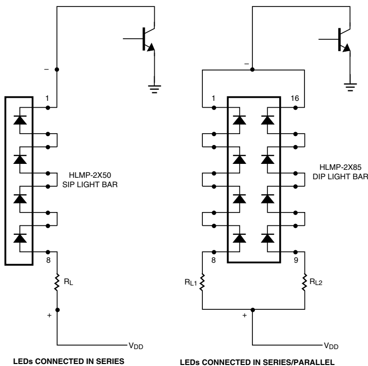
Figure 1. LED Light Bars Series, Series/Parallel Connections
