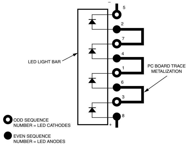
Figure 4. Alternating Pin Sequence Reduces Thermal Stress on LEDs During Hand Soldering
