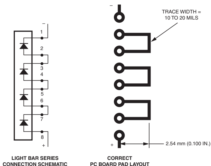
Figure 3. Trace Layout Reduces Thermal Stress on LEDs During Soldering
