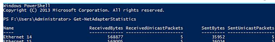
Figure 3-14 Get-NetAdapterStatistics
