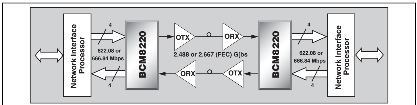
BCM8220 Application Block Diagram
