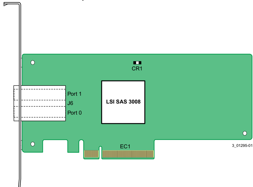
Figure 1 LSI SAS 9300-8e HBA Board Layout
