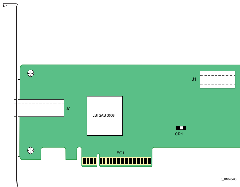
Figure 1 LSI SAS 9311-4i4e HBA Board Layout
