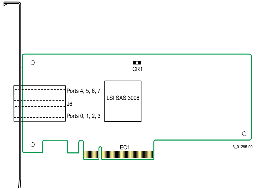
Figure 1 LSI SAS 9300-8e HBA Board Layout
