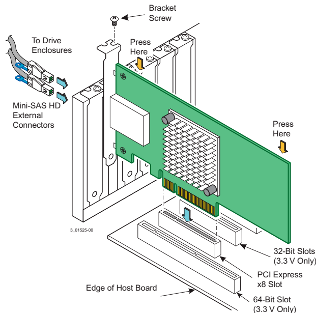
Figure 2 Install an LSI 12Gb/s x8 HBA in a PCIe Slot
