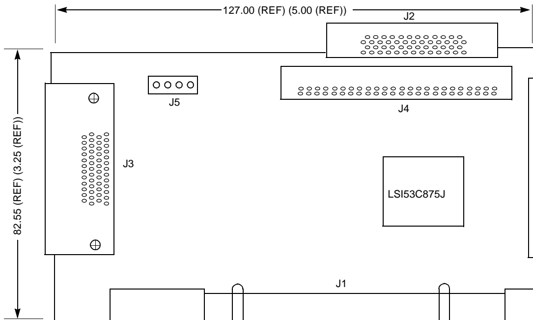
Figure A.1 LSI8751SP Mechanical Drawing
