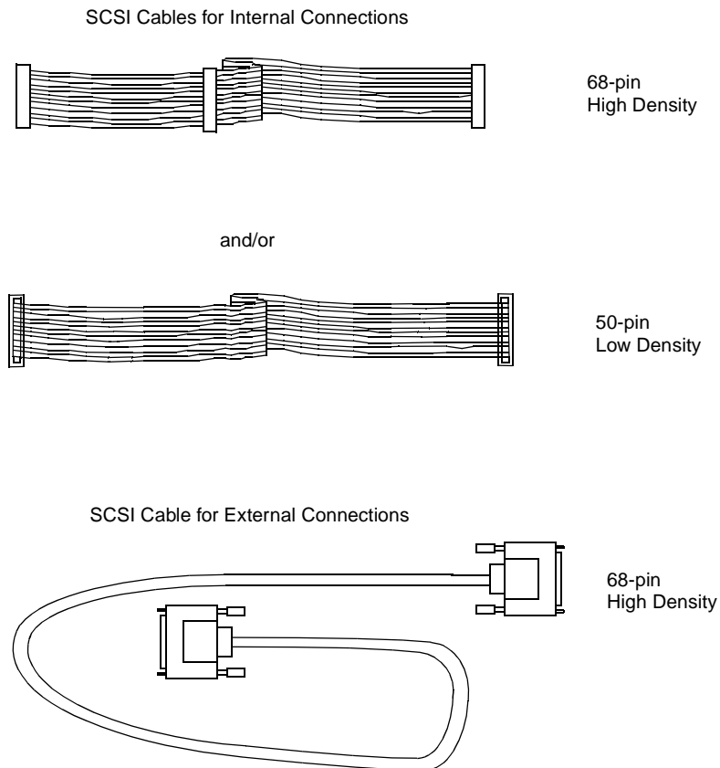
Figure 2.3 SCSI Cables
