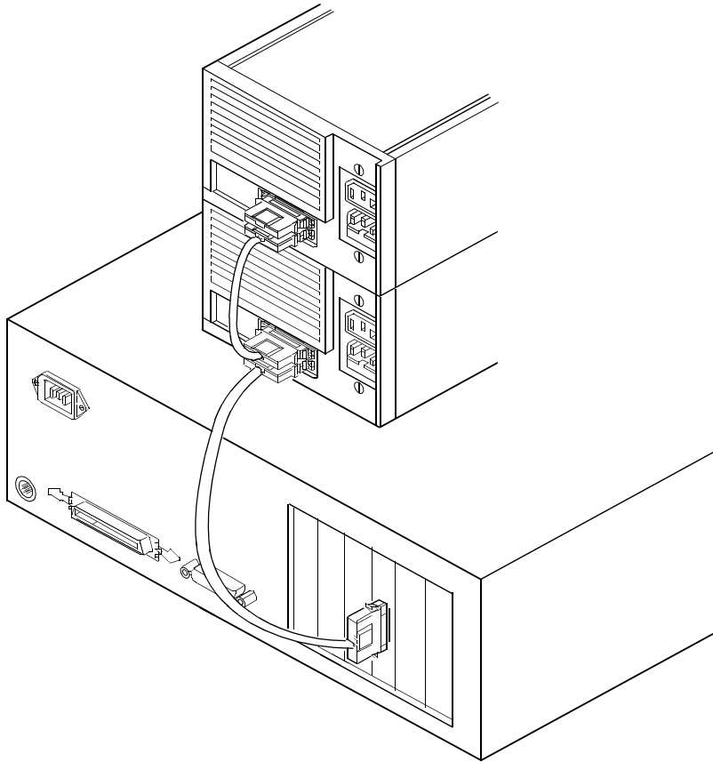
Figure 2.13 Multiple External SCSI Devices Chained Together
