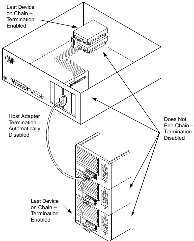
Figure 2.16 Internal and External SCSI Device Termination
