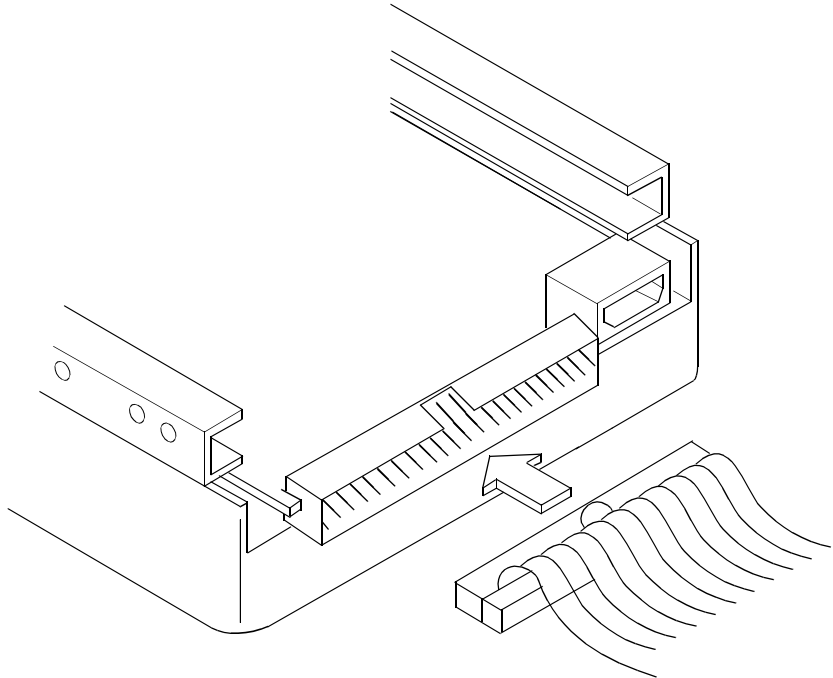
Figure 2.6 Internal SCSI Ribbon Cable to Internal SCSI Device Connection
