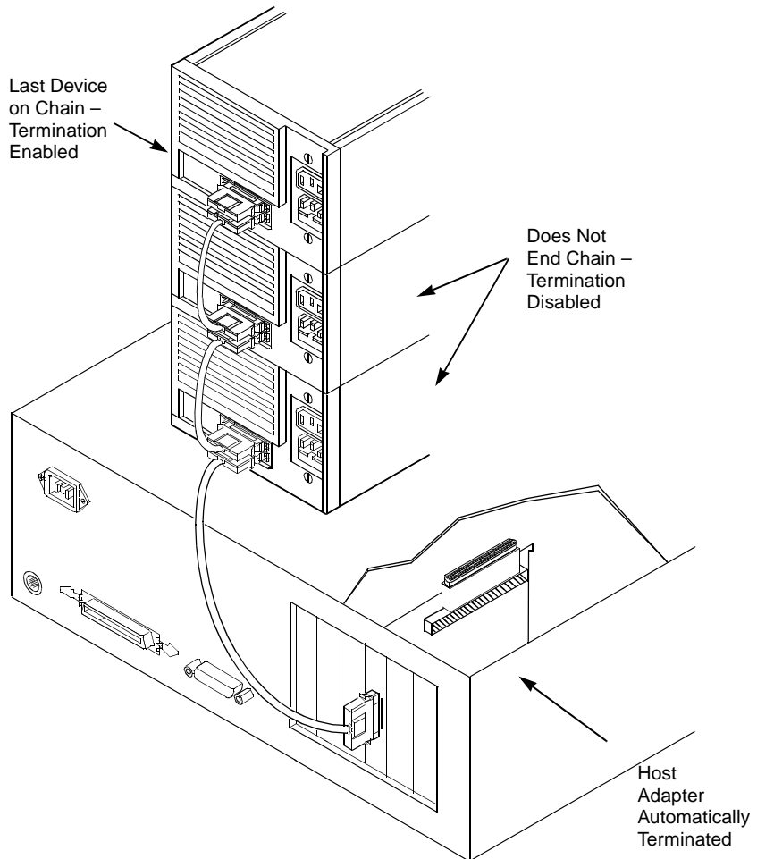
Figure 2.15 External SCSI Device Termination
