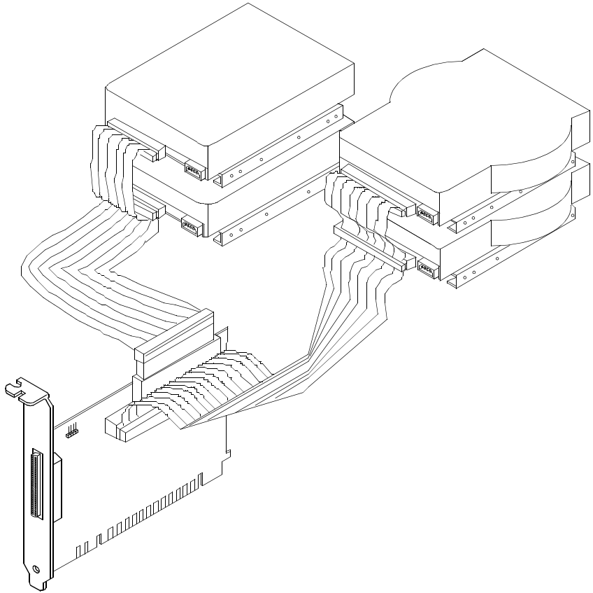
Figure 2.9 Using Both Internal Connectors
