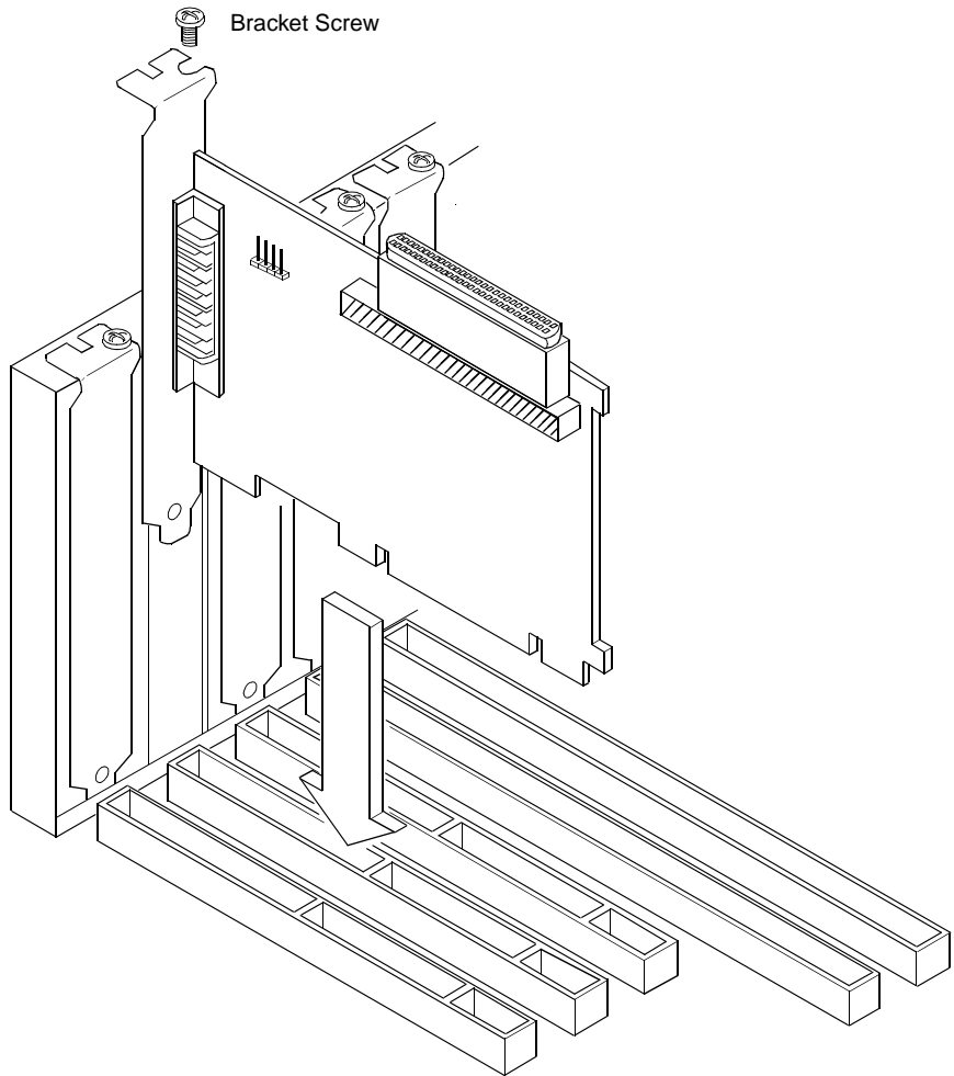
Figure 2.2 Inserting the Host Adapter
