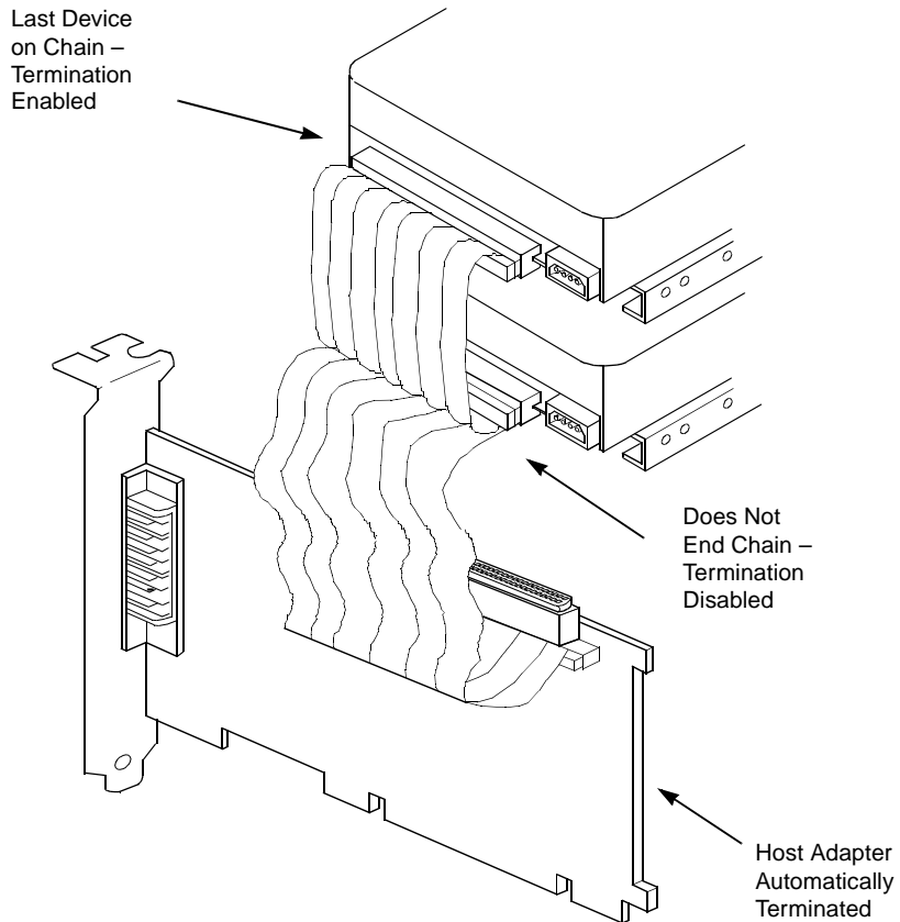
Figure 2.14 Internal SCSI Device Termination
