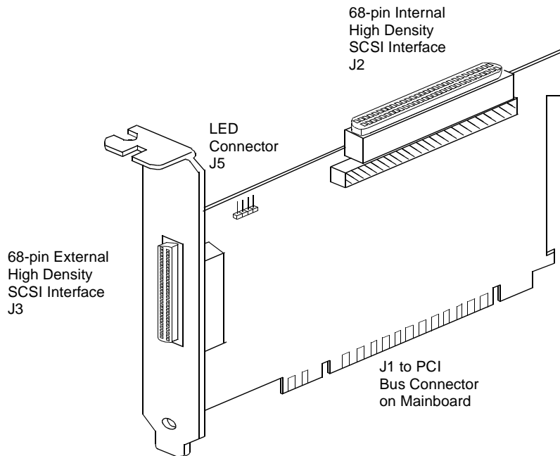
Figure 2.1 Hardware Connections for the LSI8751SP
