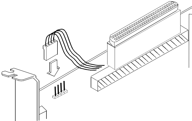
Figure 2.10 SCSI LED Connector
