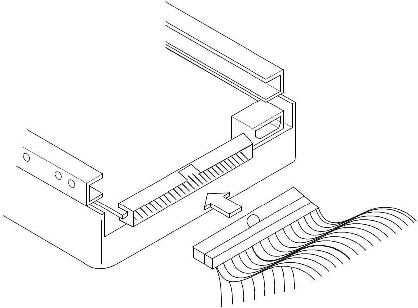
Figure 2.7 Connection Additional Internal SCSI Devices
