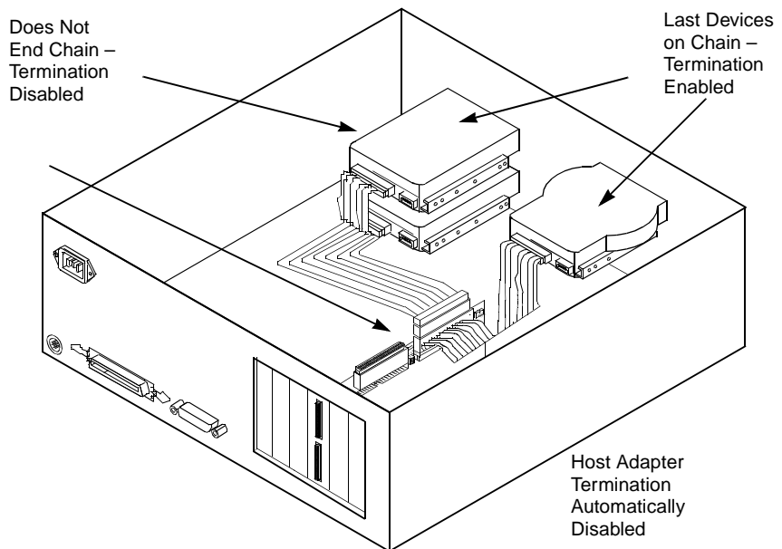
Figure 2.17 Internal and Internal SCSI Device Termination
