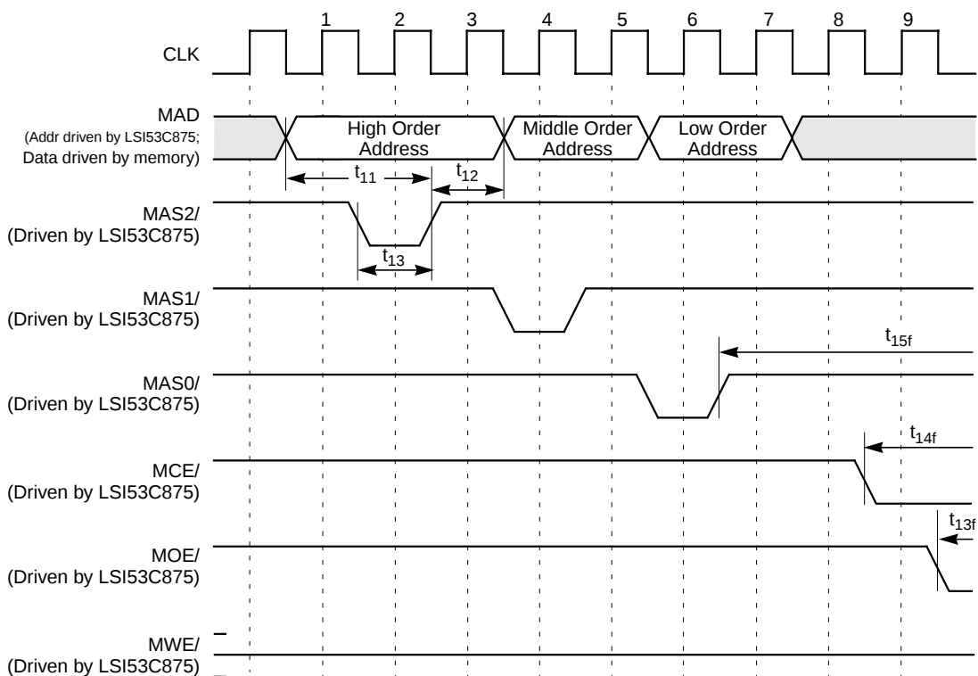
Figure 7.21 Read Cycle, Normal/Fast Memory ( \geq 64 Kbytes), Single Byte Access
