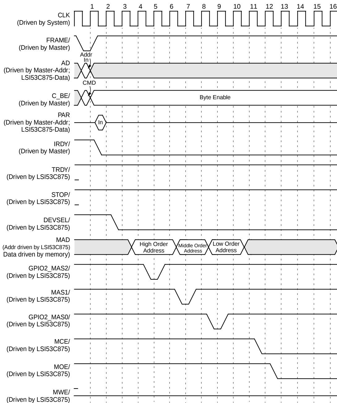
Figure 7.23 Read Cycle, Normal/Fast Memory ( \geq 64 Kbyte), Multiple Byte Access
