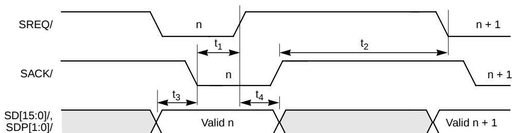
Figure 7.35 Initiator and Target Synchronous Transfer
