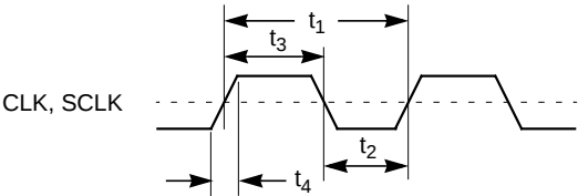
Figure 7.6 Clock Waveforms
