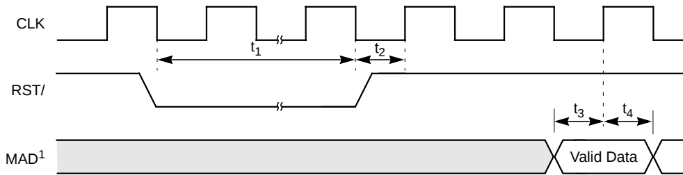
Figure 7.7 Reset Input
