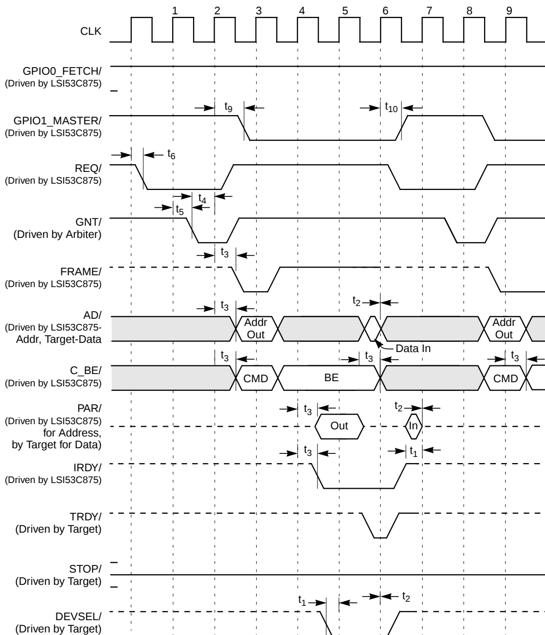
Figure 7.19 Burst Read
