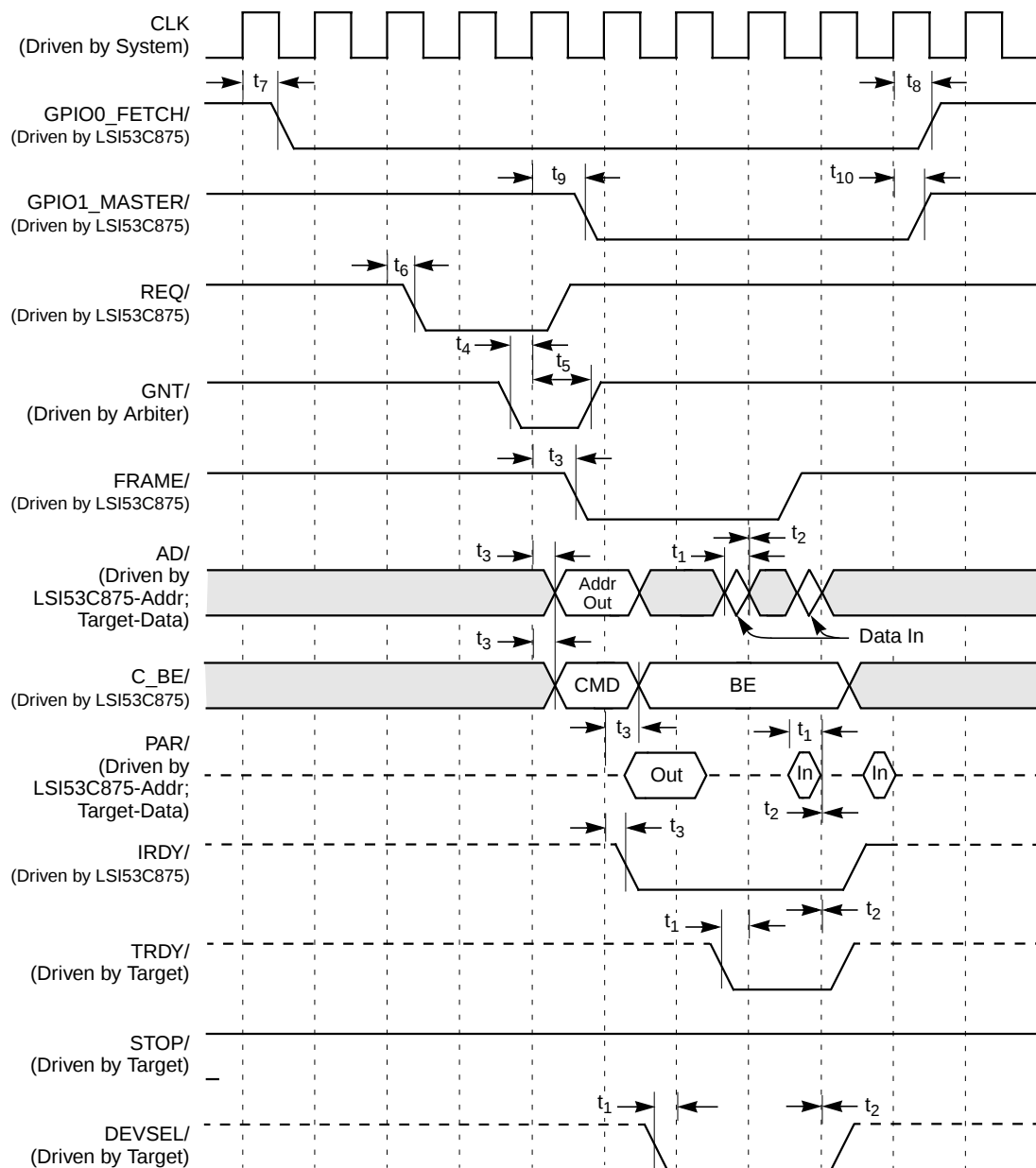
Figure 7.16 Burst Opcode Fetch
