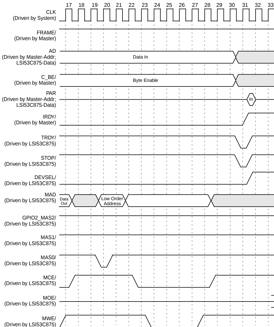
Figure 7.24 Write Cycle, Normal/Fast Memory ( \geq 64 Kbyte), Multiple Byte Access (Cont.)
