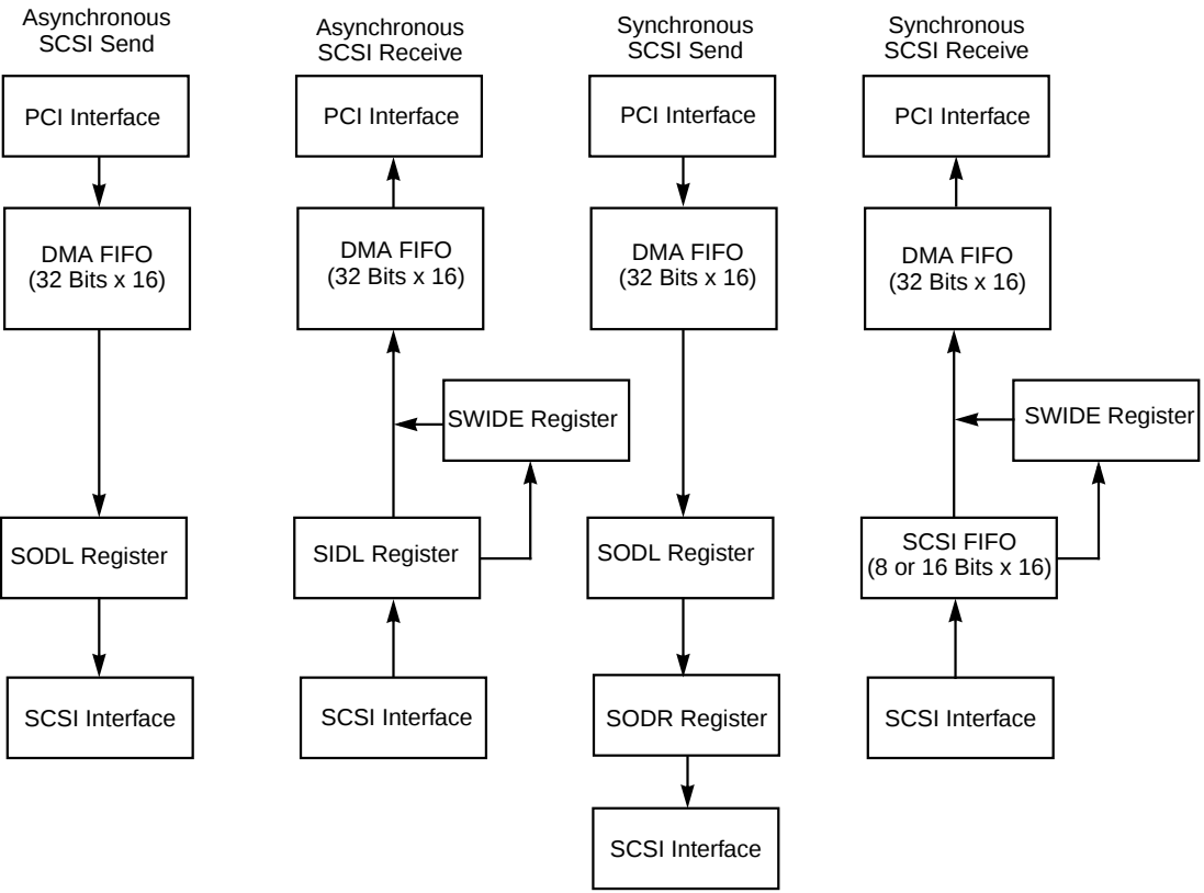
Figure 2.2 LSI53C875 Host Interface Data Paths
