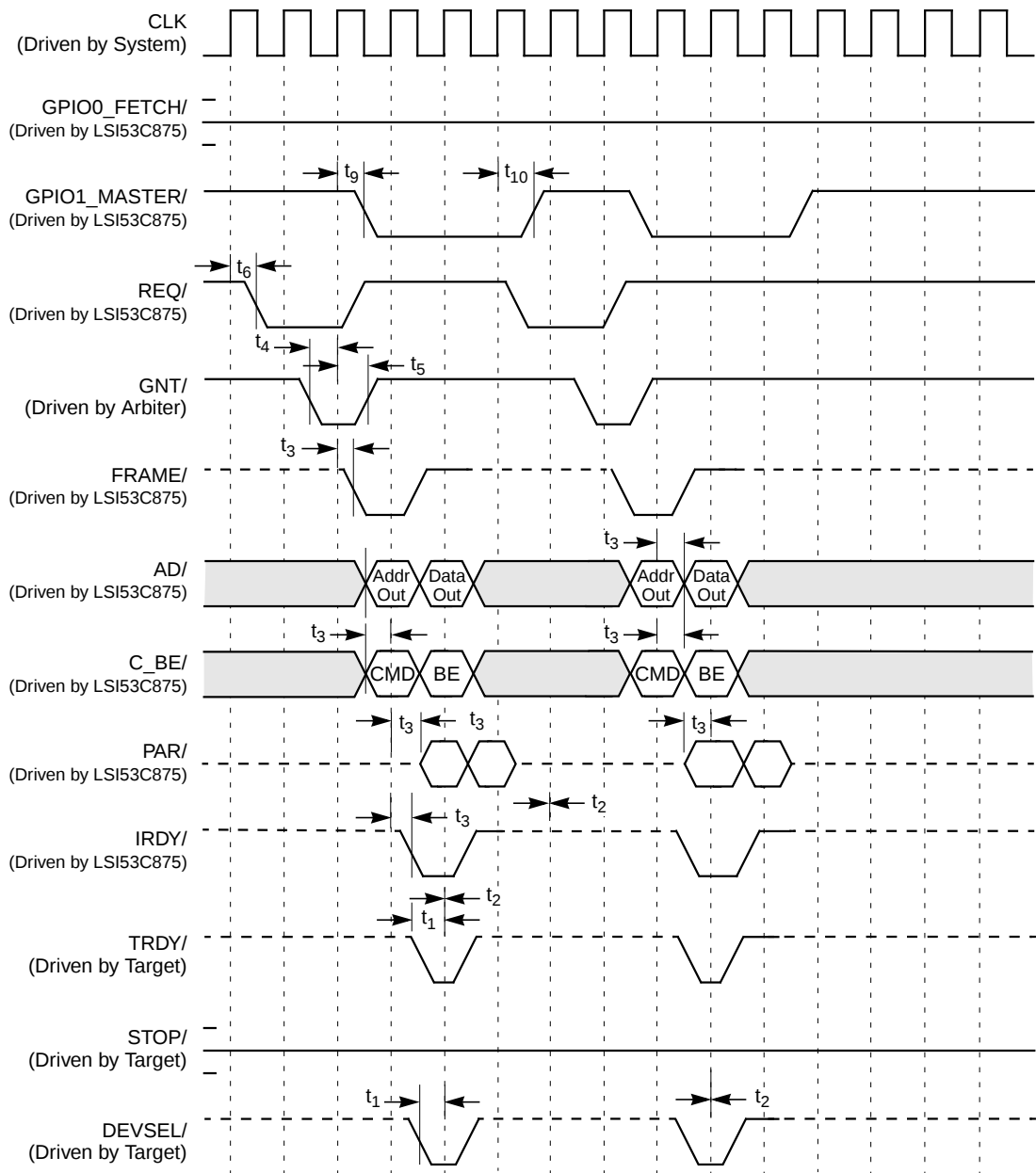
Figure 7.18 Back-to-Back Write
