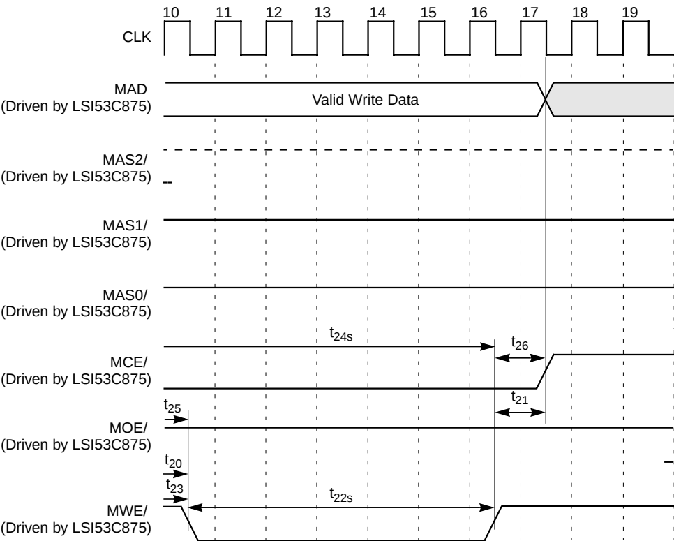
Figure 7.30 Write Cycle, Slow Memory ( \leq 64 Kbyte) (Cont.)
