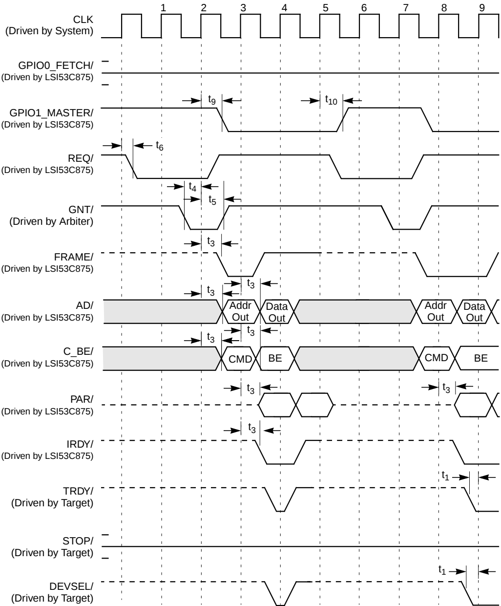
Figure 7.20 Burst Write
