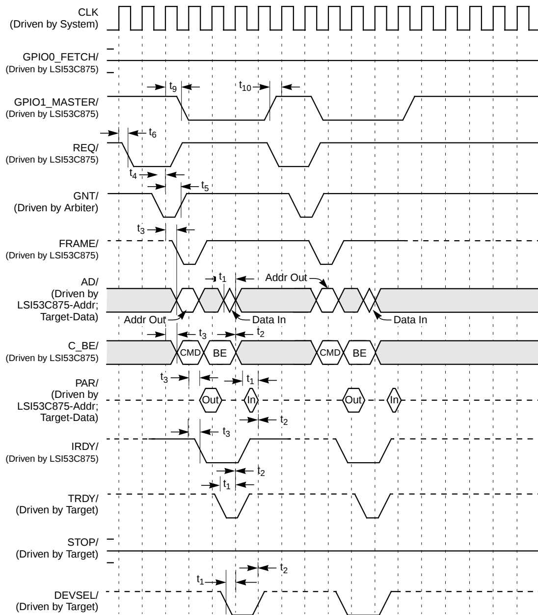
Figure 7.17 Back-to-Back Read
