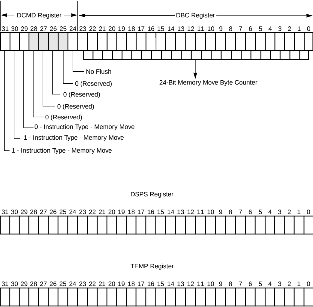
Figure 6.6 Memory Move Instruction
