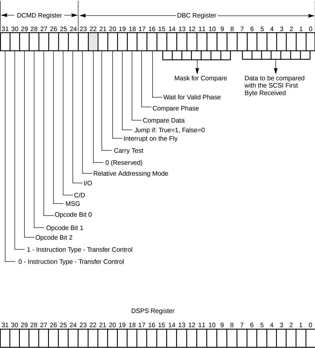
Figure 6.5 Transfer Control Instructions
