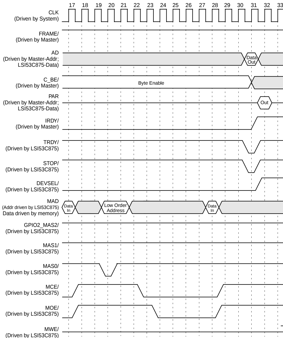
Figure 7.23 Read Cycle, Normal/Fast Memory ( \geq 64 Kbyte), Multiple Byte Access (Cont.)
