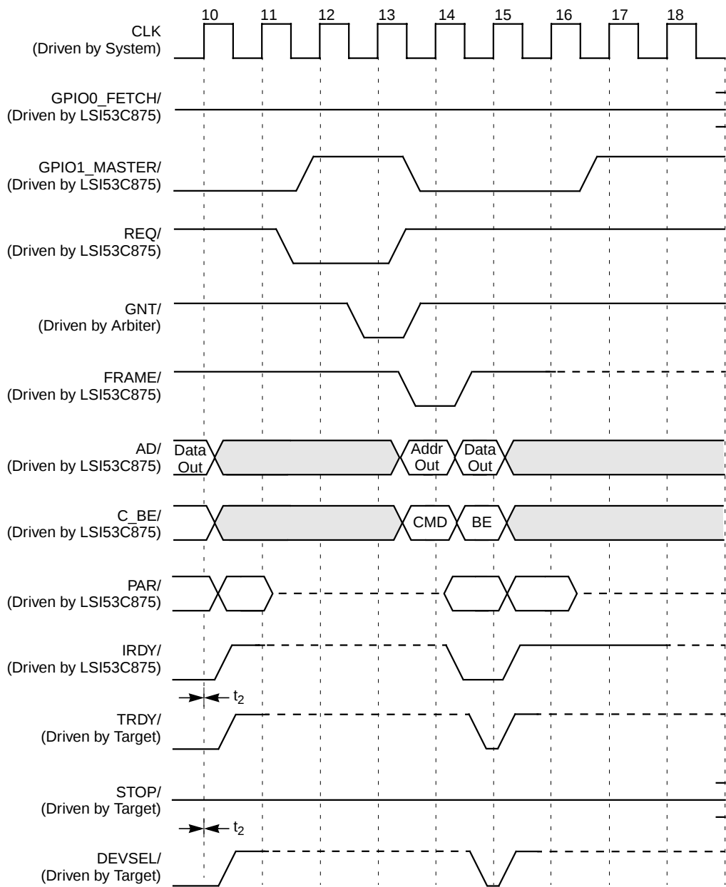
Figure 7.20 Burst Write (Cont.)
