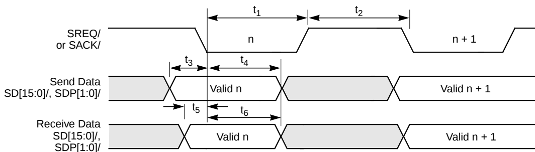
Figure 7.35 Initiator and Target Synchronous Transfer
