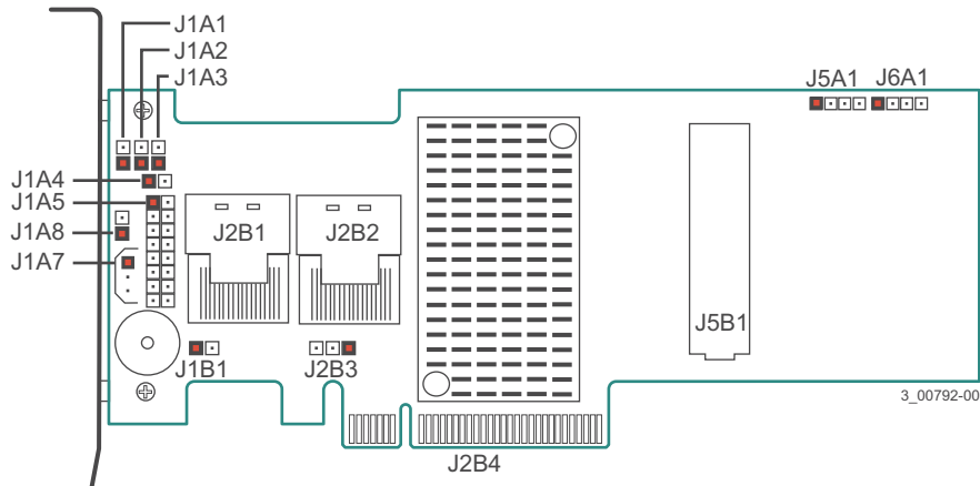
Figure 15 Card Layout for the MegaRAID SAS 9265CV-8i RAID Controller
