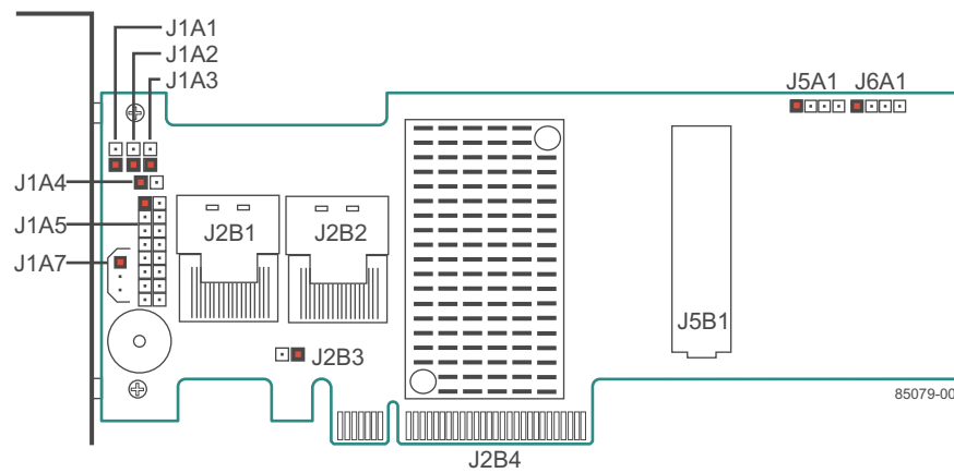
Figure 14 Card Layout for the MegaRAID SAS 9265-8i RAID Controller
