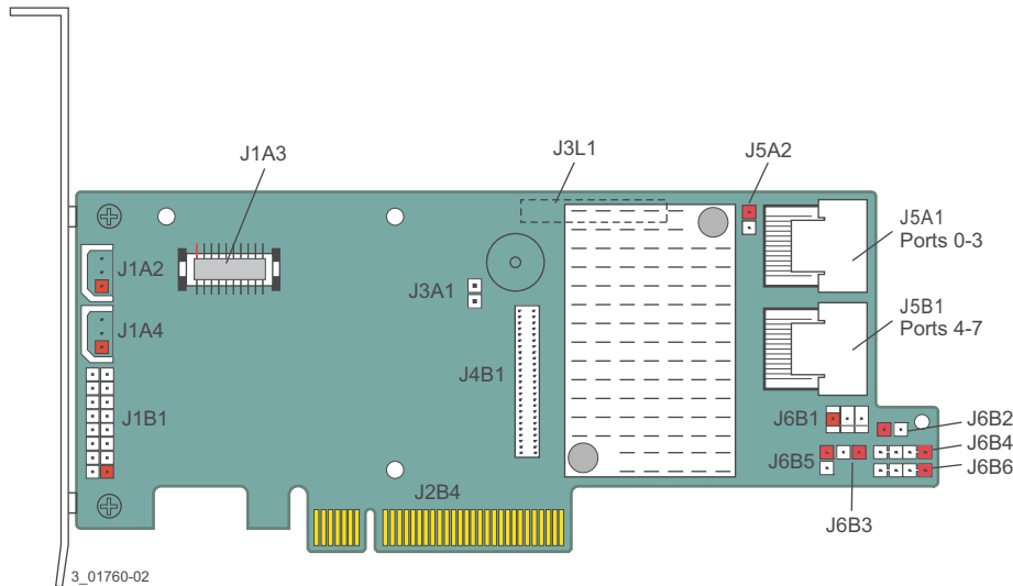
Figure 18 Card Layout for the MegaRAID SAS 9271-8i RAID Controller
