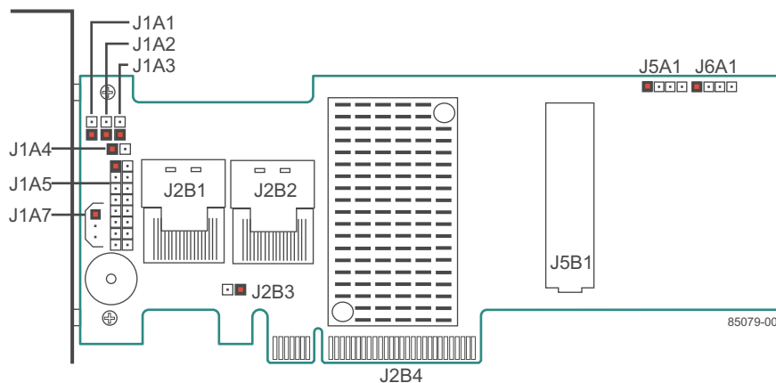
Figure 17 Card Layout for the MegaRAID SAS 9270-8i RAID Controller
