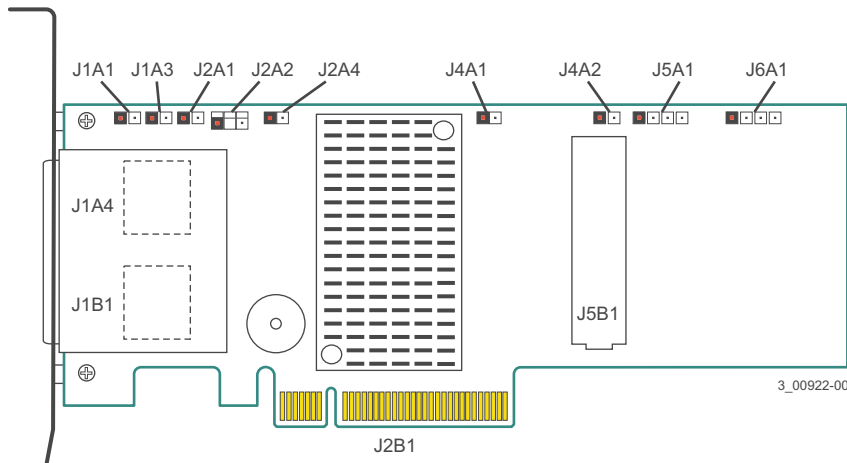
Figure 25 Card Layout for the MegaRAID SAS 9286CV-8e RAID Controller
