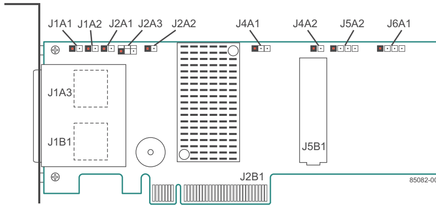
Figure 24 Card Layout for the MegaRAID SAS 9286-8e RAID Controller
