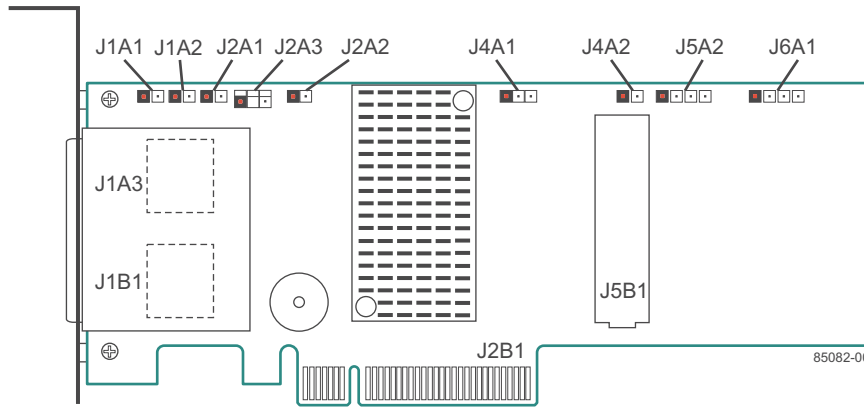
Figure 22 Card Layout for the MegaRAID SAS 9285-8e RAID Controller
