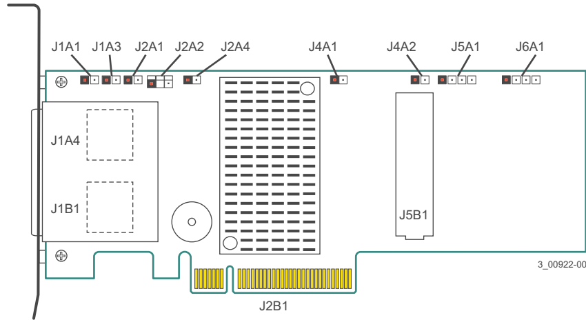
Figure 23 Card Layout for the MegaRAID SAS 9285CV-8e RAID Controller
