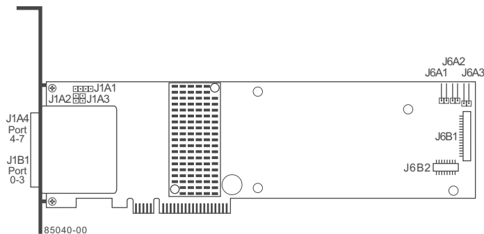
Figure 19 Card Layout for the MegaRAID SAS 9280-8e RAID Controller
