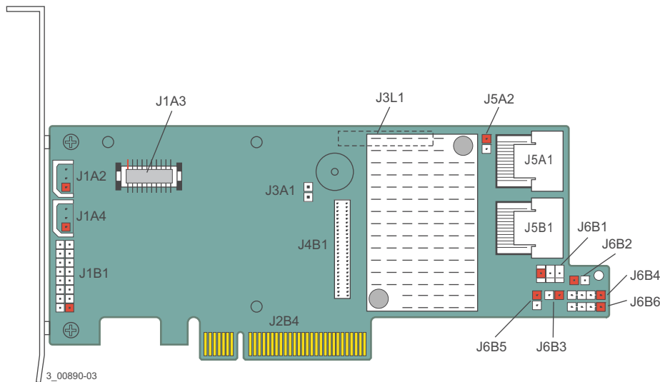
Figure 16 Card Layout for the MegaRAID SAS 9266-8i RAID Controller
