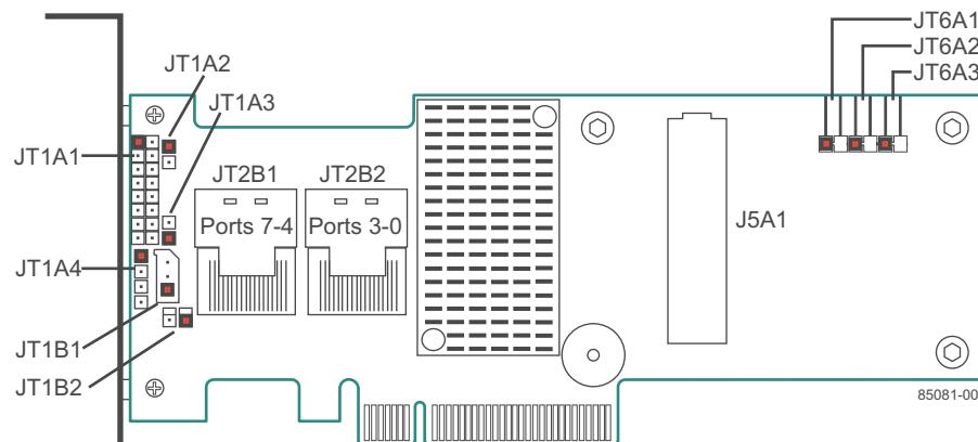
Figure 12 Card Layout for the MegaRAID SAS 9260CV-8i RAID Controller
