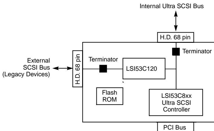
Figure 1.4 SCSI Bus Electrical Isolation
