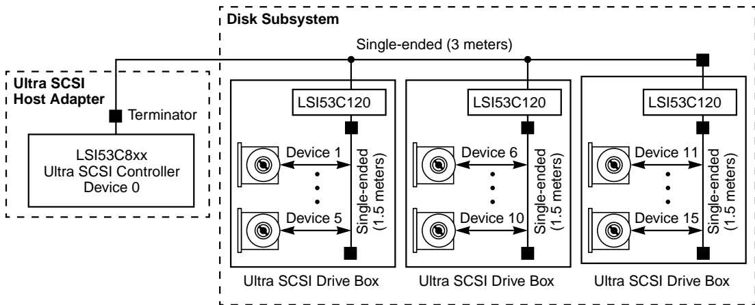
Figure 1.2 SCSI Extender Application (SE to SE Mode of Operation)
