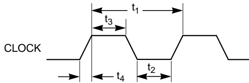
Figure 3.8 Clock Timing
