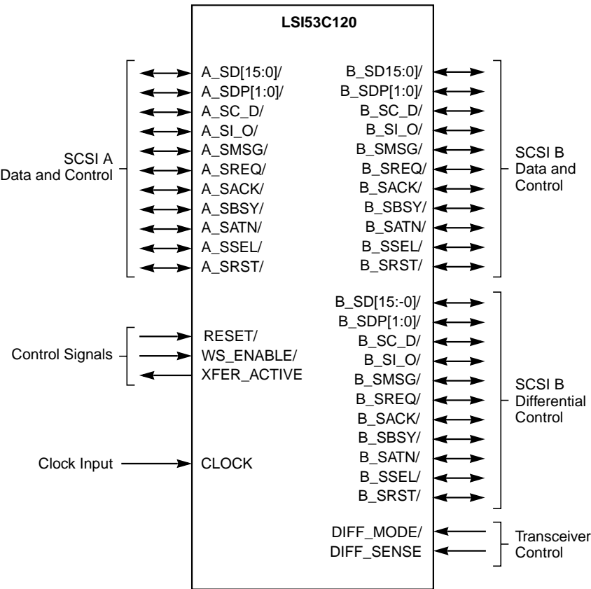
Figure 3.2 LSI53C120 Functional Signal Grouping
