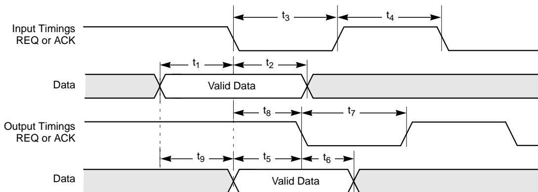
Figure 3.9 Input/Output Timing
