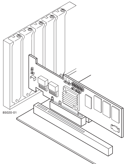
Figure 2 Installing the MegaRAID SAS 8708EM2 RAID Controller
