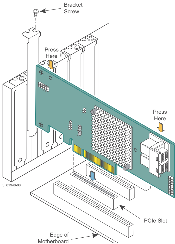
Figure 1 Installing the MegaRAID SAS 9341-8i RAID Controller
