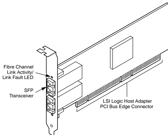
Figure 2 LSI7202XP-LC Fibre Channel Cable Connections
