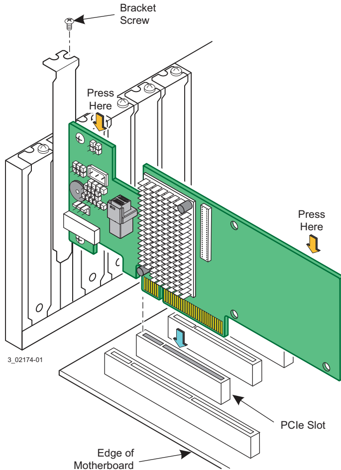
Figure 1 Installing the MegaRAID SAS 9380-4i4e RAID Controller
